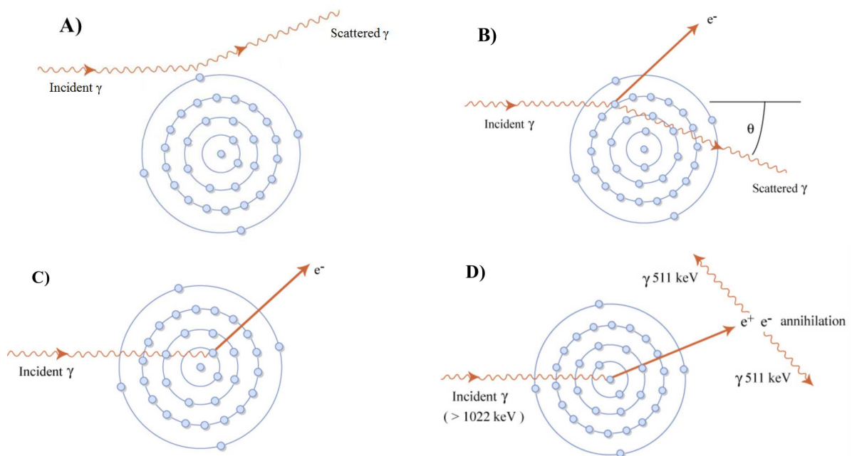
Figure 1.6: Schemes of the principal phenomena of photon interaction with matter: A) Rayleigh scattering, B) Compton scattering, C) Photoelectric effect, D) Pair Production [13].
