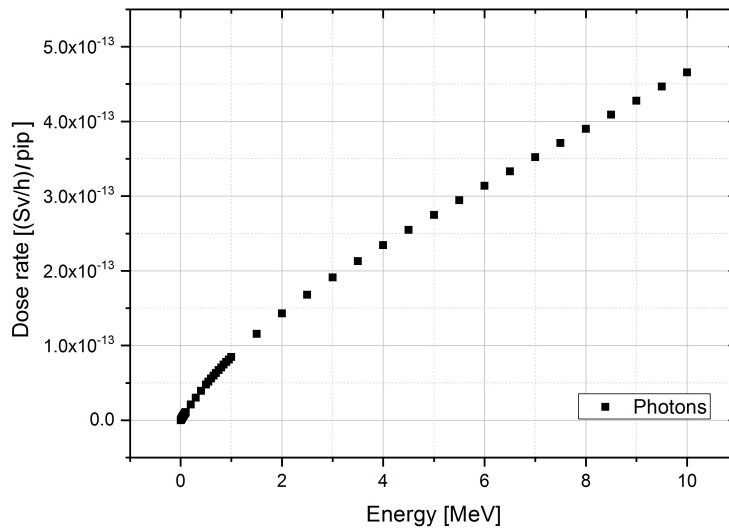
Figure 4.4: Dose rate results of MCNPX simulations for monoenergetic gamma sources. The range of simulated energies goes from 0.01 to 10 MeV.
