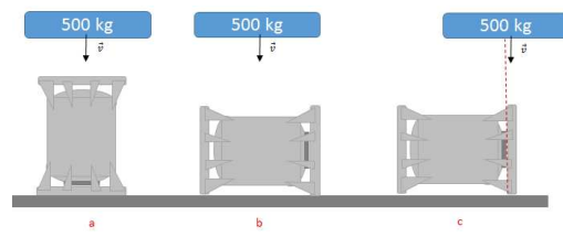
Figure 2.54: Scheme of the dynamic drop test, drop of 500 kg on the package.
