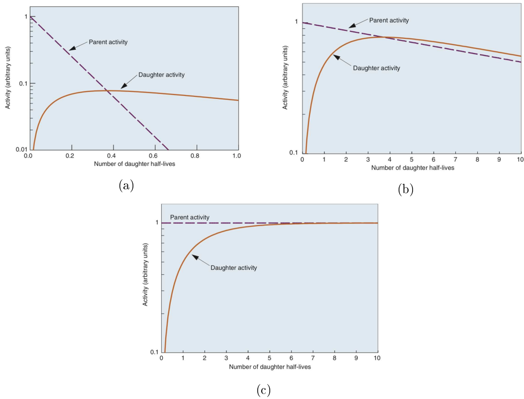
Figure 1.4: Types of parent-daughter nuclide equilibrium. a) No equilibrium, b) transient equilibrium, c) secular equilibrium [13].
