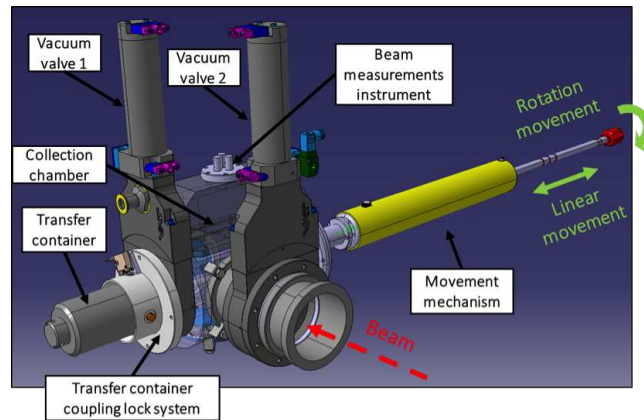
Figure A.6: 3D drawing of the actual Isotope collection system in MEDICIS [drawing: S.Marzari, CERN].
