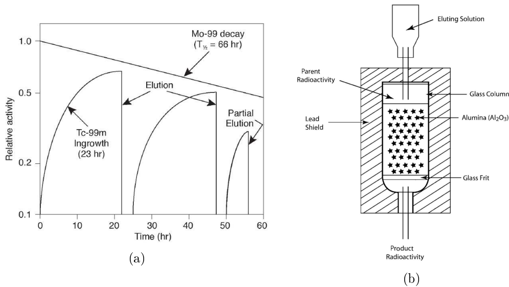
Figure 1.5: a) Regeneration of the Tc-99m at each elution within 23h, time to obtain the max Tc-99 activity. b) Schematics of a generator [20].
