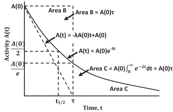
Figure 1.3: Activity A(t) plotted versus time t for a simple decay of a radioactive parent P into its daughter D [20].
