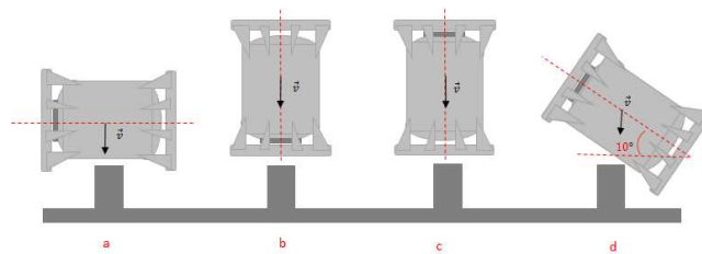
Figure 2.47: Scheme of the drop test of a rigid bar.
