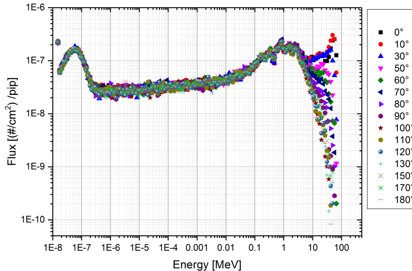
Figure 3.19: Results of the MCNPX simulation for neutrons (top: liner scale, bottom: log-log scale).
