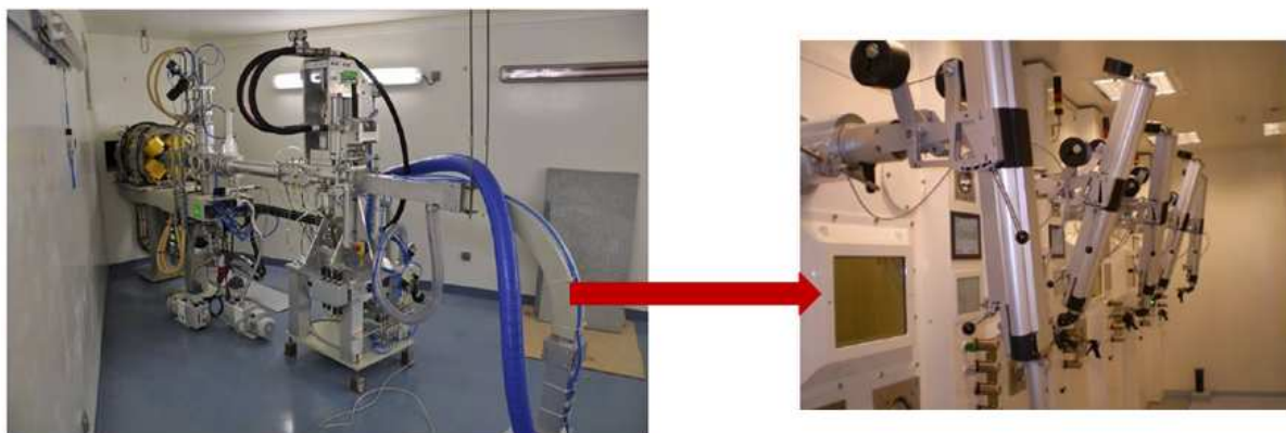
Figure 3.6: Photo of the Irradiation bunker A1 (left) and of the connected hot cells (right) for the target dismantling.
