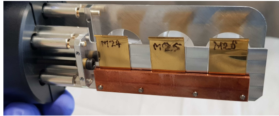
Figure A.4: Gold foils used for the collection in MEDICIS [photo: R. Formento].
