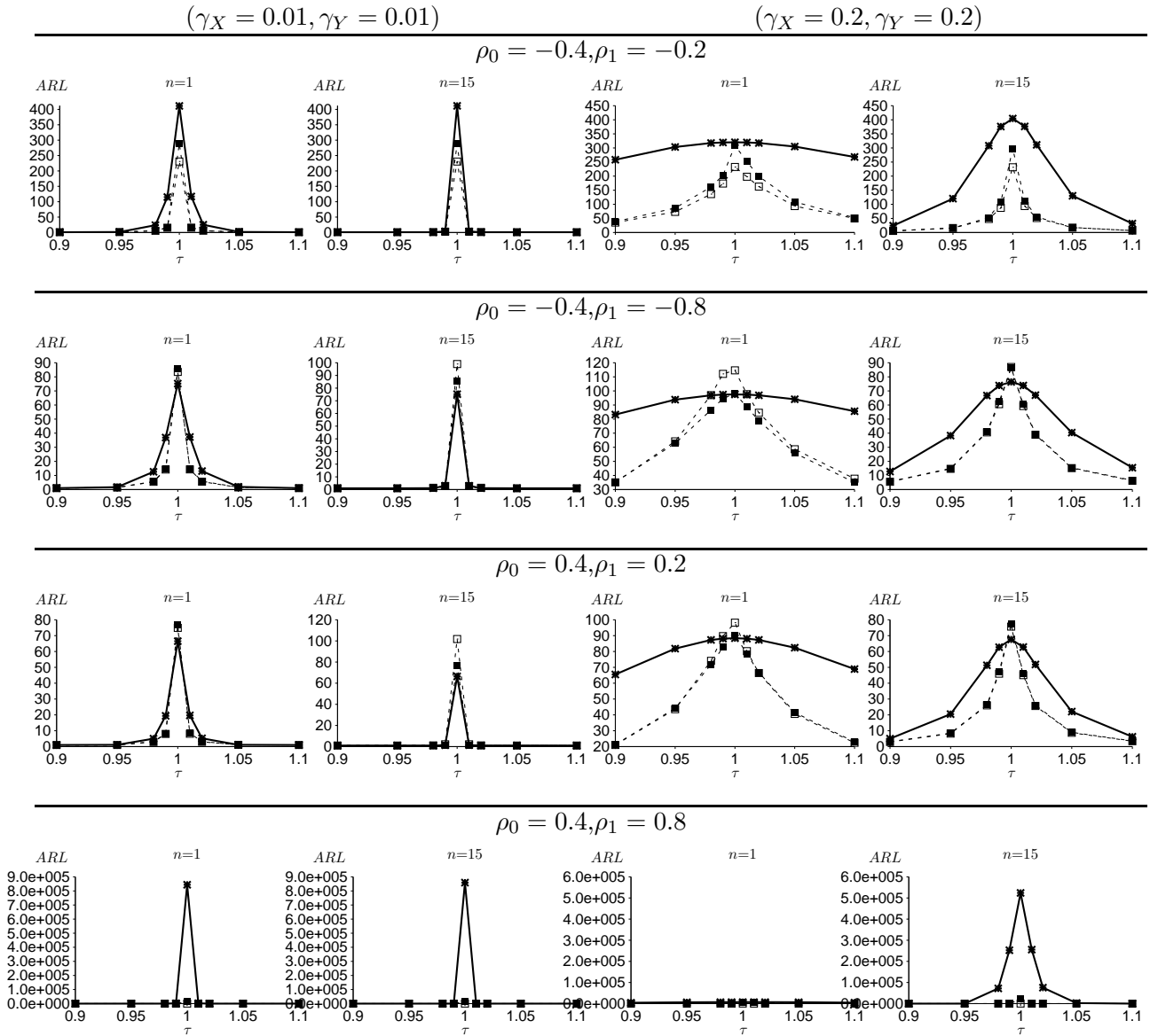
FIGURE 5.4 : Valeurs de ARL_1 pour les cartes CUSUM-RZ ( -\square- ), EWMA-RZ ( -\blacksquare- ) et Shewhart-RZ ( -*- ) pour \gamma_X \in \{0.01, 0.2\} , \gamma_Y \in \{0.01, 0.2\} , \gamma_X = \gamma_Y , (\rho_0, \rho_1) = \{(-0.4, -0.2), (-0.4, -0.8), (0.4, 0.2), (0.4, 0.8)\} , \tau \in \{0.90, 0.95, 0.98, 0.99, 1.01, 1.02, 1.05, 1.10\} , n \in \{1, 15\} et ARL_0 = 200
