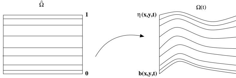
FIGURE 4.3 – Example of a discrete sigma-transform
