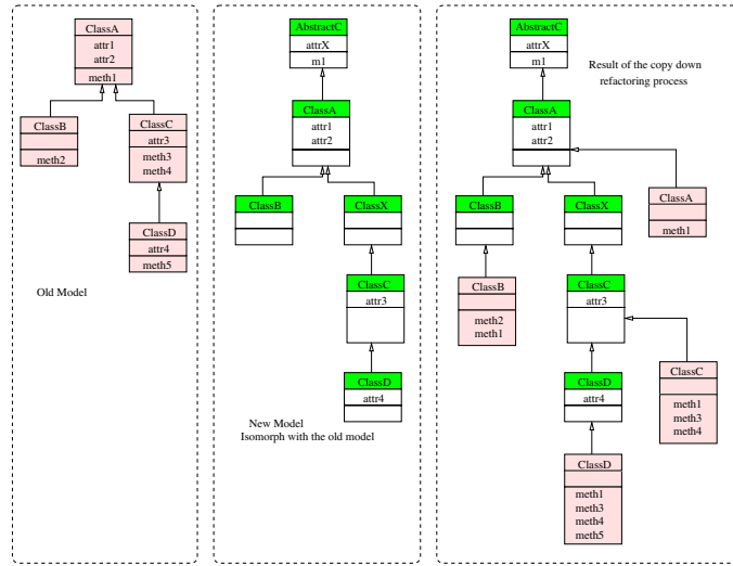
Figure 4.22: Example model transformation using CopyDown method
