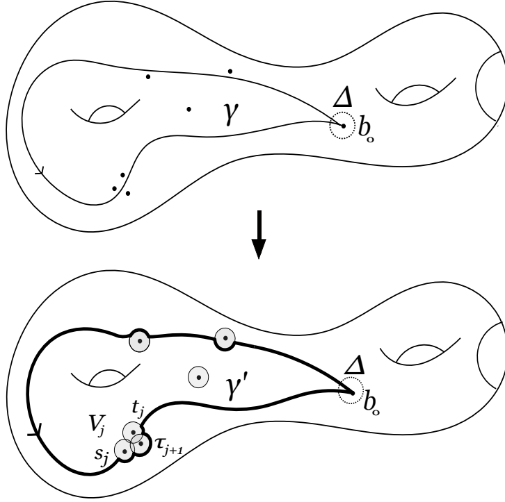
FIGURE 5.1. Procedure (*) applied to \gamma (with \Delta = V(b_0, a/s) )
