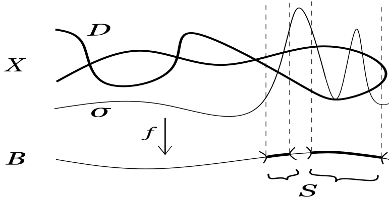
FIGURE 1.1. An (S, \mathcal{D}) -integral section \sigma
