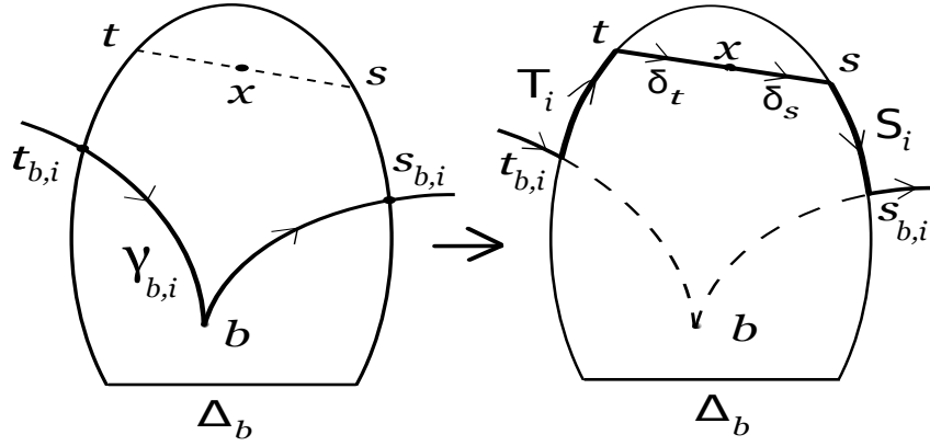
FIGURE 5.2. Local modification of \gamma_{b,i} \cap \Delta_b
