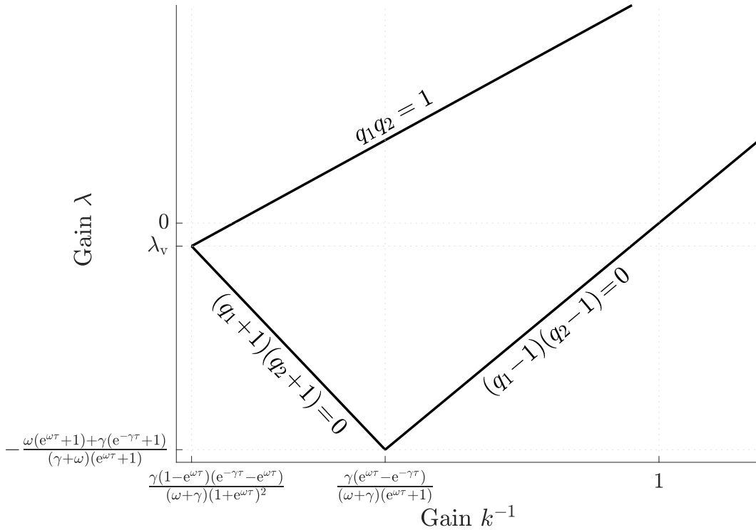
Figure 3.3: Set of stable gains for P_d \rightarrow \mathbf{X}P . The set of feedback gains k^{-1} and \lambda that lead to a stable closed-loop dynamics is a triangle, where \lambda varies between -\frac{\omega(e^{\omega\tau}+1)+\gamma(e^{-\gamma\tau}+1)}{(\gamma+\omega)(1+e^{\omega\tau})} and \frac{\omega(e^{\omega\tau}-1)+\gamma(e^{-\gamma\tau}-1)}{(\gamma+\omega)(1-e^{\omega\tau})} while k^{-1} varies between \frac{\gamma(1-e^{\omega\tau})(e^{-\gamma\tau}-e^{\omega\tau})}{(\gamma+\omega)(1+e^{\omega\tau})^2} and \frac{\gamma(e^{-\gamma\tau}-e^{\omega\tau})}{(\gamma+\omega)(1-e^{\omega\tau})} . \lambda_v has a long expression, it can be positive or negative depending on the parameters \gamma, \omega, \tau .
