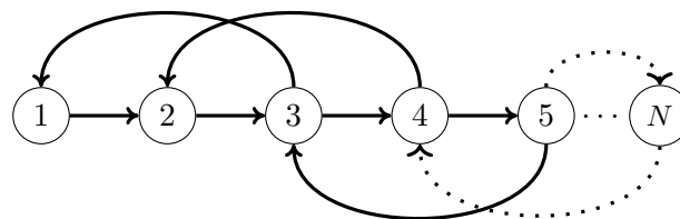
Figure 5.11 – Entangled cycles
