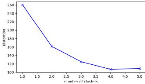
(a) Elbow method.
