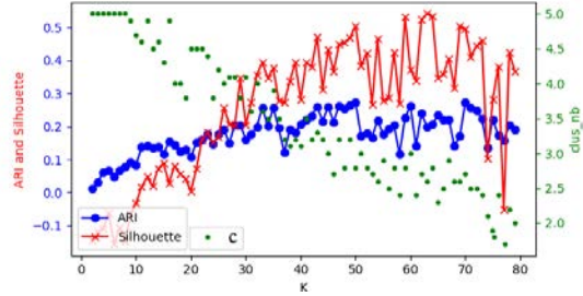
(b) ARI, silhouette coefficient and number of clusters vs. k .
