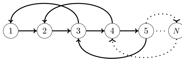
Figure 5.11 – Entangled cycles
