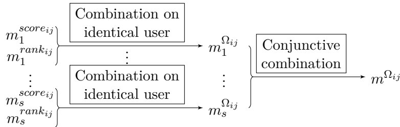
Figure 6.5 – Combination procedure for sushi preferences
