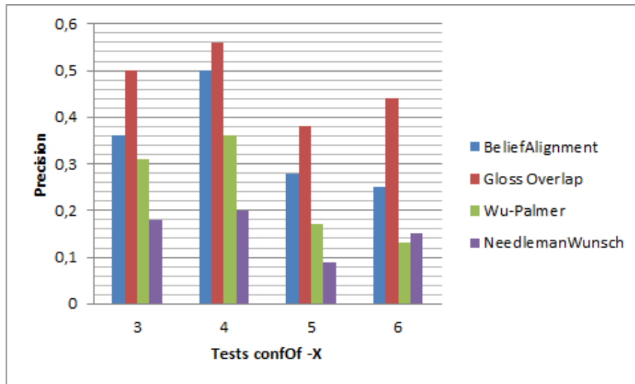
Figure 4.8: Precision results between ConfOf and X
