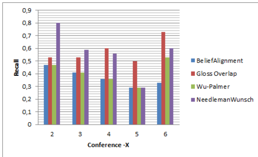
Figure 4.7: Recall results between Conference and X
