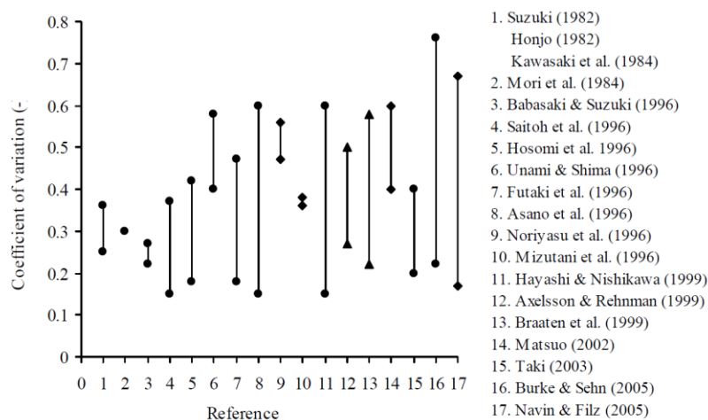
Figure 1-14 Coefficient of variation evaluated from compression tests in a number of reported studies (Larsson, 2005).
