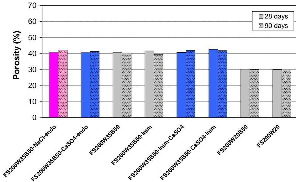
Figure 5-22 Effect of CaSO 4 and NaCl on the total porosity of Fontainebleau sand-CEM III cement mixes.
