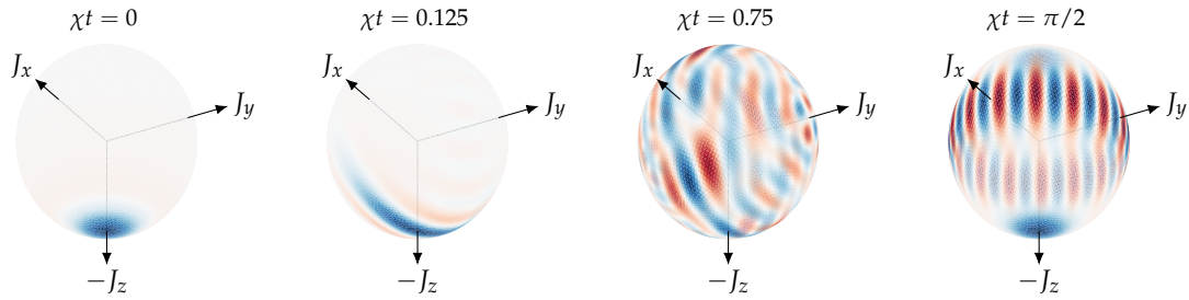
Figure 4.10 – One-axis twisting evolution: Wigner distributions. We show the Wigner distribution (bottom view) from the initial state ( \chi t = 0 ) up to the N00N state at ( \chi t = \pi/2 ), with intermediate times for a spin squeezed state ( \chi t = 0.125 ) and a ‘dephased’ state ( \chi t = 0.75 ).
