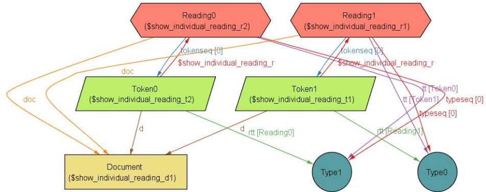
Figure 3.2: An instance of the transcription model with possible individual readings.
