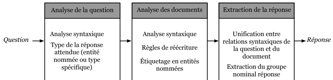
FIGURE 4.1: Architecture de FIDJI
