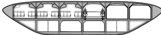
Figure 1.17: Integrated cabin structure design.
