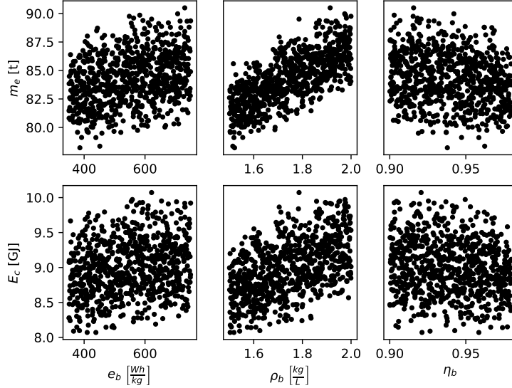
Figure 3.15: Effects on OWE m_e and energy consumption E_c of battery technology parameters. Fixed battery case.
