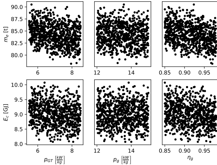
Figure D.2: Effects on OWE m_e and energy consumption E_c of gas turbine and generator technology parameters for the hybrid aircraft case, R = 900 nmi, N_{EM} = 32 . Fixed battery case.
