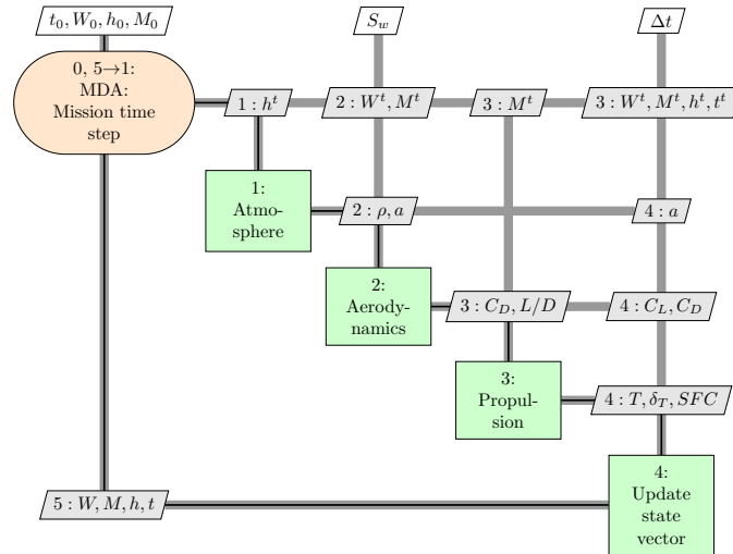
Figure 2.5: xDSM diagram for the time step performance analysis.
