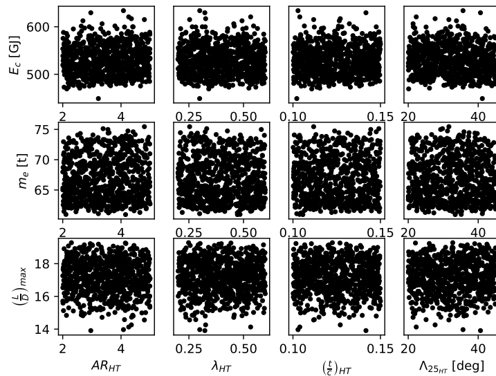
Figure D.10: Effect of HT parameters over energy consumption E_c , OWE m_e and maximum LoD for the hybrid aircraft case, R = 900 nmi, N_{EM} = 32 .
