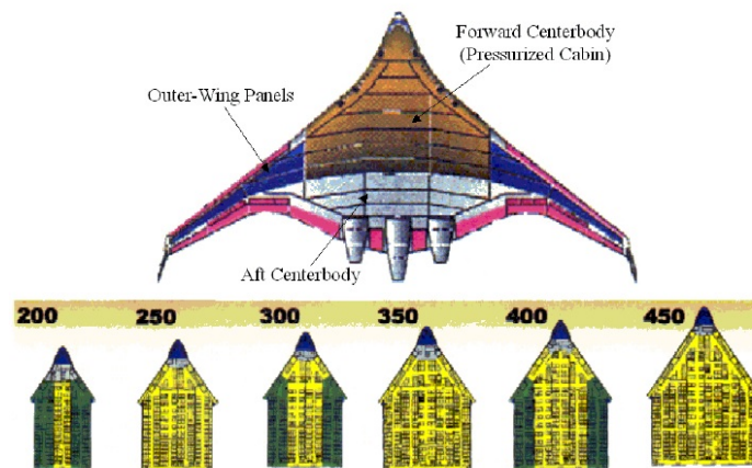
Figure 1.20: Blended Wing-Body cabin design, according to Bradley [Bra04]
