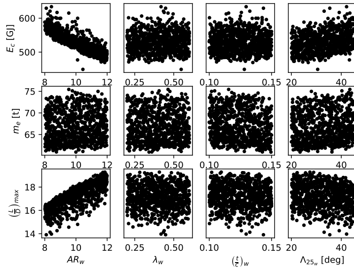
Figure D.9: Effect of wing parameters over energy consumption E_c , OWE m_e and maximum LoD for the hybrid aircraft case, R = 900 nmi, N_{EM} = 32 .
