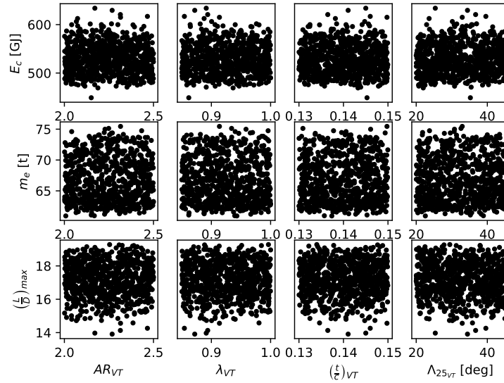
Figure D.11: Effect of VT parameters over energy consumption E_c , OWE m_e and maximum LoD for the hybrid aircraft case, R = 900 nmi, N_{EM} = 32 .
