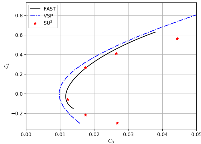
Figure 4.5: C_D - C_L curve, comparison between SU2, FAST and OpenVSP. RANS simulation case M=0.78 and h=35000\text{ft} .
