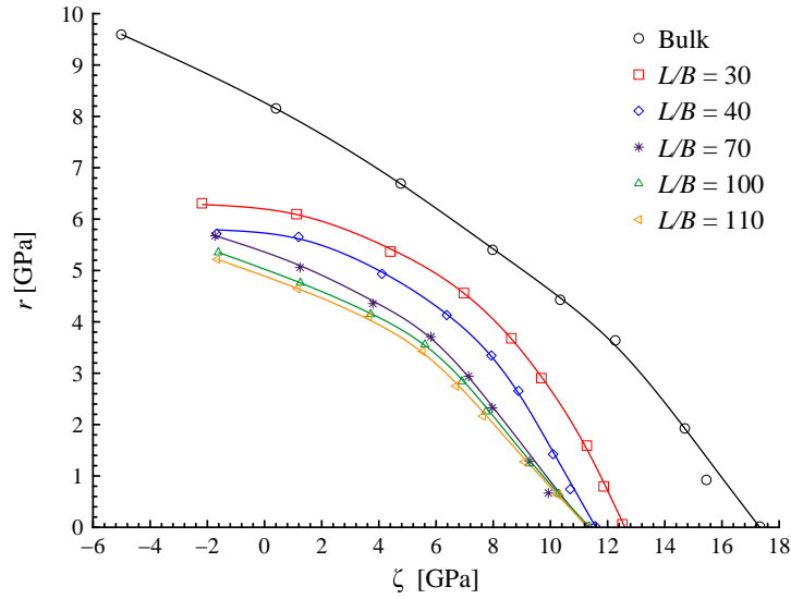
Figure 2.11 – Nanovoiced sample ( p = 1\% ). Numerical results (symbols) and estimated meridian strength profiles for different values of L/B and for a \text{TXE}_\Sigma state ( \theta_\Sigma = 0 ). The bulk case is also reported.
