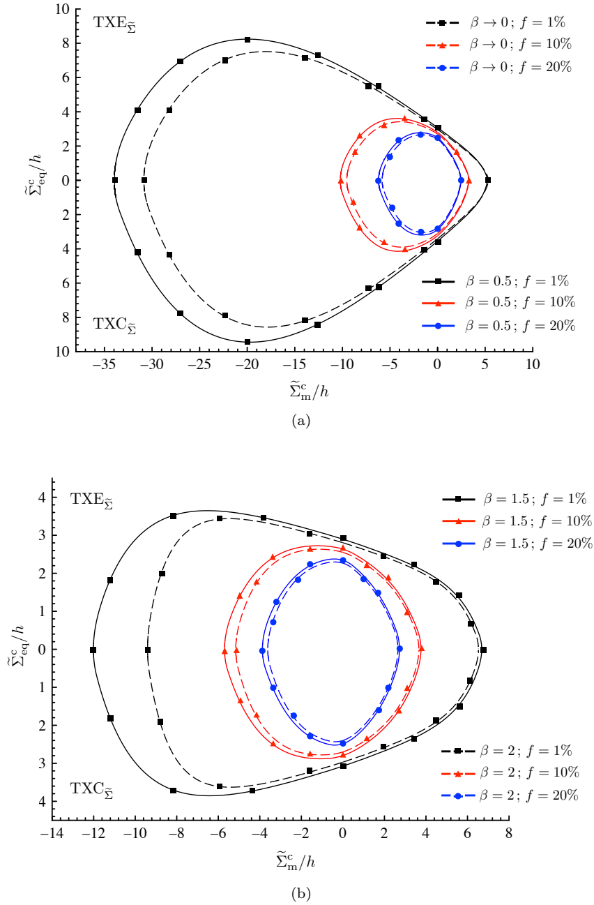
Figure 4.7 – Hollow-sphere model without interface effects (that is, for \kappa \rightarrow 0^+ ). Triaxial-expansion ( \text{TXE}_{\tilde{\Sigma}} ) and triaxial-compression ( \text{TXC}_{\tilde{\Sigma}} ) strength profiles for different values of parameter \beta and porosity f . Local plastic behaviours complying with: (a) (\xi, \beta) \in \mathcal{N} for \xi = 2\xi^{**} ; (b) (\xi, \beta) \in \mathcal{O} for \xi = 6\Xi^- .
