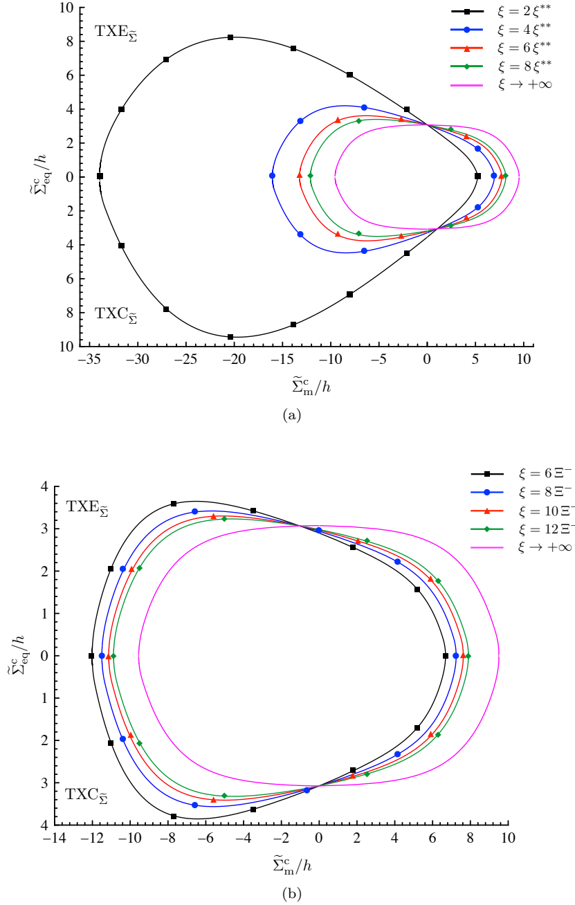
Figure 4.11 – Hollow-sphere model without interface effects (that is, for \kappa \rightarrow 0^+ ). Triaxial-expansion ( \text{TXE}_{\tilde{\Sigma}} ) and triaxial-compression ( \text{TXC}_{\tilde{\Sigma}} ) strength profiles for different values of parameter \xi , porosity being set equal to f = 1\% . Local plastic behaviours complying with: (a) (\xi, \beta) \in \mathcal{N} for \beta = 0.5 ; (b) (\xi, \beta) \in \mathcal{O} for \beta = 1.5 .
