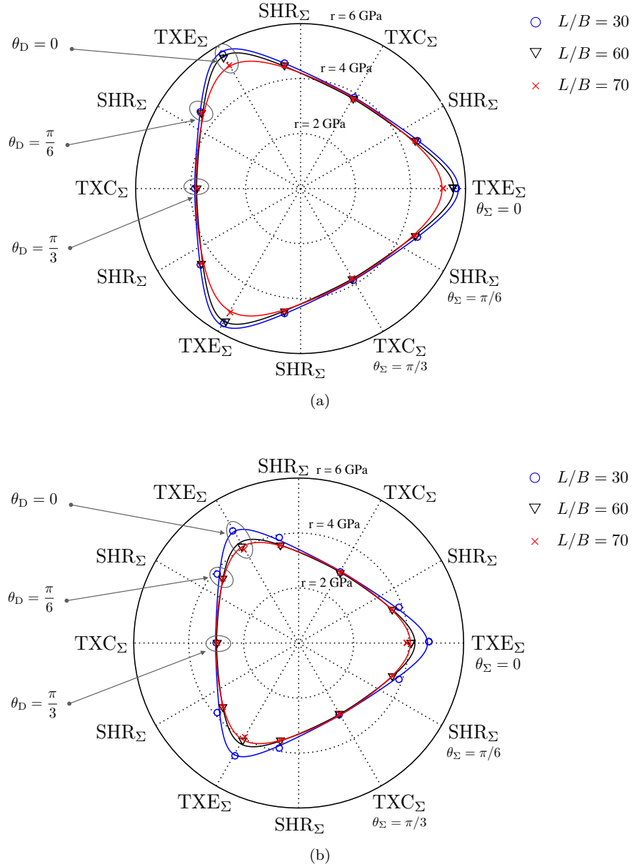
Figure 2.13 – Nanovoided sample ( p = 0.5\% ). Numerical results (symbols) and estimated deviatoric strength profiles in the \pi -planes for different values of L/B . (a) \zeta = 2 GPa. (b) \zeta = 6 GPa.
