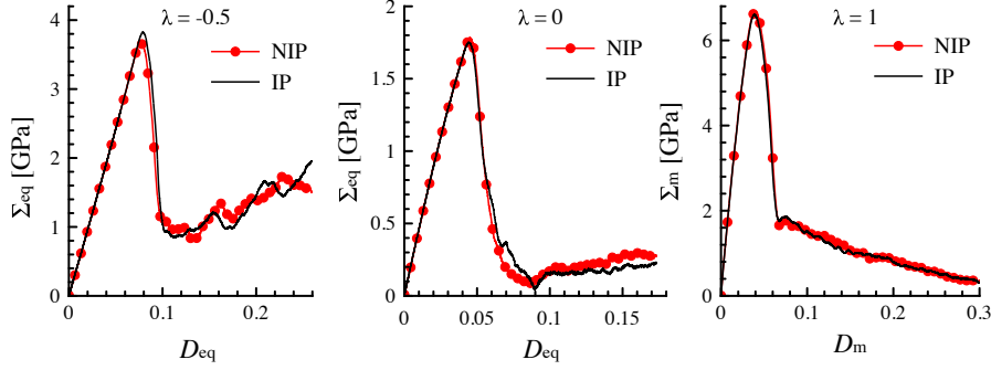
Figure 2.2 – Stress-strain relationships computed for the deformation path \text{TXE}_D with: \lambda = -0.5 (pure deviatoric state), \lambda = 0 (traction test) and \lambda = 1 (pure hydrostatic state). L/B = 50 , R = 1.353 \text{ nm} , p = 1\% . IP: isothermal process (at 300 K). NIP: non-isothermal process.
