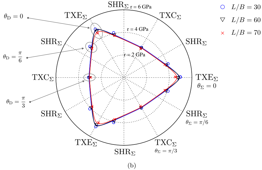
Figure 2.14 – Nanovoiced sample ( p = 0.1\% ). Numerical results (symbols) and estimated deviatoric strength profiles in the \pi -planes for different values of L/B . (a) \zeta = 2 GPa. (b) \zeta = 6 GPa.
