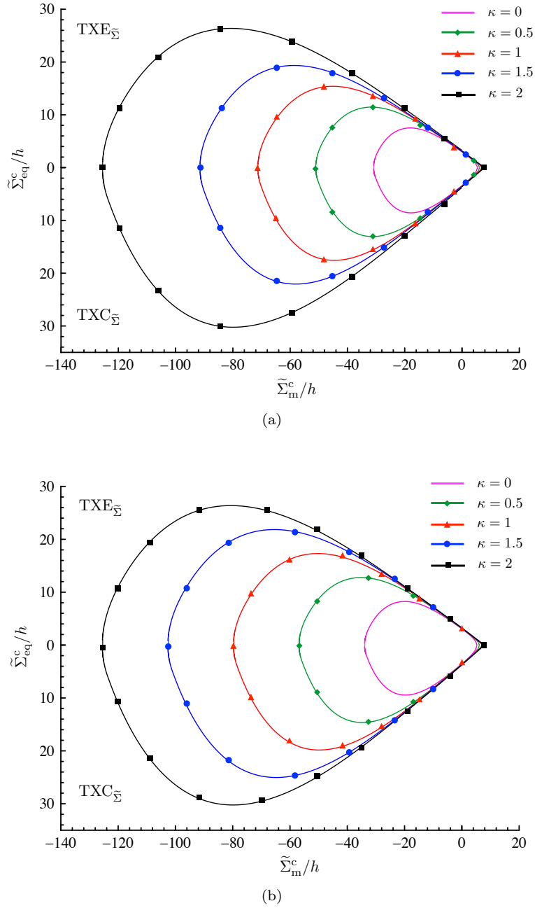
Figure 4.8 – Hollow-sphere model with interface effects. Triaxial-expansion ( \text{TXE}_{\bar{\Sigma}} ) and triaxial-compression ( \text{TXC}_{\bar{\Sigma}} ) strength profiles for different values of the void-size parameter \kappa , porosity being set equal to f = 1\% . Local plastic behaviours complying with: (a) (\xi, \beta) \in \mathcal{N} for \beta \rightarrow 0 and \xi = 2\xi^{**} ; (b) (\xi, \beta) \in \mathcal{N} for \beta = 0.5 and \xi = 2\xi^{**} .
