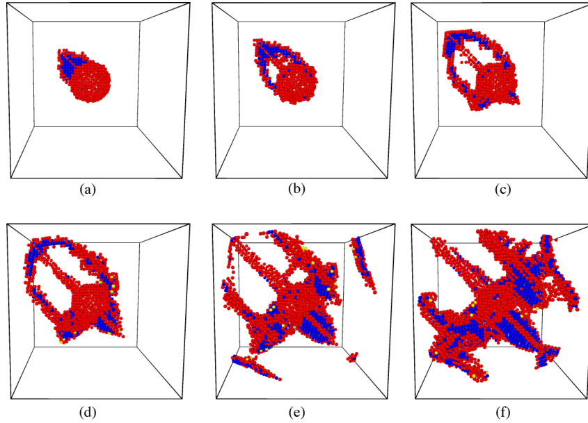
Figure 2.5 – (Top) Stress-strain relationship, temperature-strain relationship, and CNA results computed under a pure strain-based deviatoric condition corresponding to a non-isothermal deformation path \text{TXE}_D ( \lambda = -0.5 , L/B = 50 , R = 1.353 \text{ nm} , p = 1\% ). z1: elastic zone; z2: activation of plastic mechanisms; z3: stress-relaxation zone. (Bottom) Atomic patterns and CNA results corresponding to different states within zones z2 and z3. Percentages of icosahedral (ICO) and cubic diamond (DIA) atomic arrangements are equal to zero.
