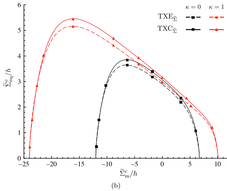
Figure 4.10 – Hollow-sphere model with interface effects. Asymmetry between triaxial-expansion ( \text{TXE}_{\tilde{\Sigma}} ) and triaxial-compression ( \text{TXC}_{\tilde{\Sigma}} ) strength profiles for different values of the void-size parameter \kappa , porosity being set equal to f = 1\% . Local plastic behaviours complying with: (a) (\xi, \beta) \in \mathcal{N} for \beta = 0.5 and \xi = 2\xi^{**} ; (b) (\xi, \beta) \in \mathcal{O} for \beta = 1.5 and \xi = 6\xi^- .
