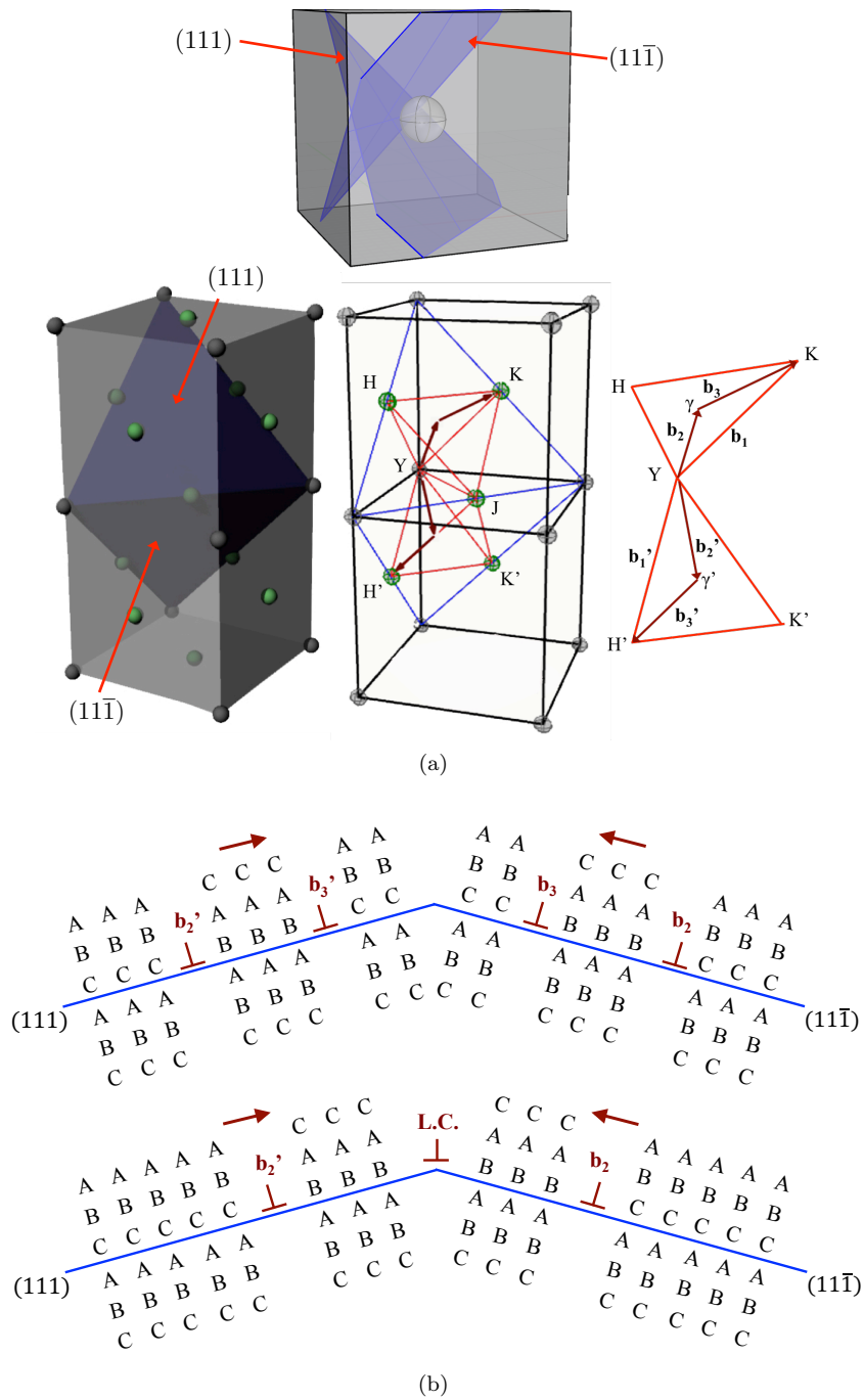
Figure 2.16 – (a) An example of Shockley-partials nucleation. Perfect dislocations b_1 and b_1' dissociate into partials, namely leading partials b_3 and b_3' , and trailing partials b_2 and b_2' . (b) Leading partials b_3 and b_3' modify the local stacking sequence of closed packed planes \{111\} from FCC (sequence ABC-ABC) into HCP (sequence AB-AB). On the contrary, trailing partials b_2 and b_2' remove the fault, restoring the original FCC lattice. L.C.: Lomer-Cottrell lock.
