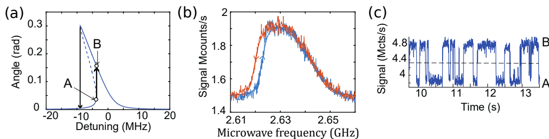
Figure 4.7: a) Expected bistable behaviour: the continuous line shows stable angular position as a function of the detuning from the magnetic resonance. For a range of parameters, two stable sites exist (eg A and B). b) Mechanically detected magnetic resonance realized by sweeping towards higher (blue) and lower (red) frequencies. c) Trace of the signal measuring the angular position under a strong red-detuned microwave.
