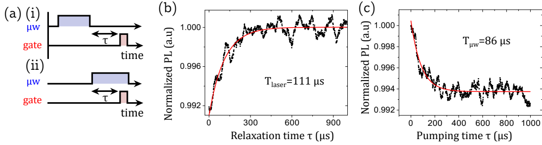
Figure 4.4: a) Sequences used to measure the time necessary for the spins' population to reach their steady states when a resonant microwave is turned (i) off and (ii) on. b) Polarization time of the spins in the non-magnetic bright state. c) Polarization time of the spins in the magnetic dark state under continuous microwave pumping (0 dBm). Curves are fitted by an exponential decay.
