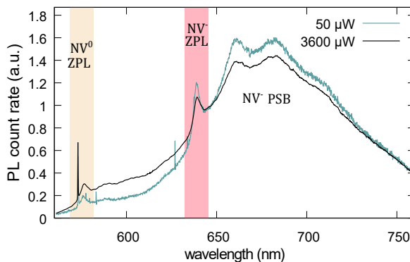
Figure 3.3: Photoluminescence spectrum of an ensemble of NV centers within a 10 \mu\text{m} diamond, deposited on a quartz coverslip under green laser excitation, for two different powers. Both features of the NV^- and NV^0 can be distinguished: the Zero Phonon Line (ZPL) and the Phonon SideBand (PSB). The sharp peak on the left of the NV^0 ZPL is Raman scattering of the green laser by the diamond.
