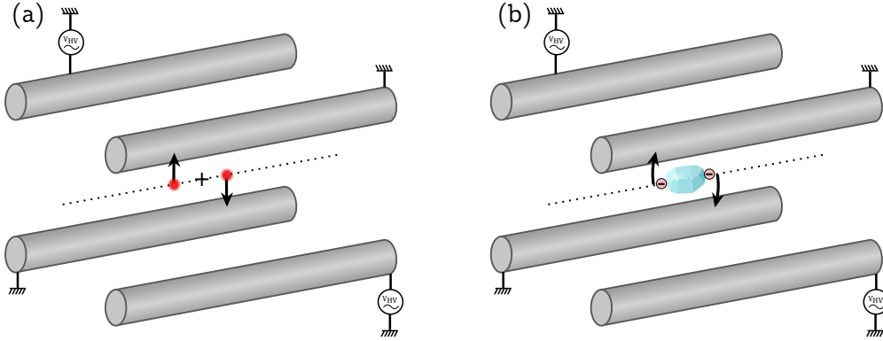
Figure 2.3: a) Ion trap with four rods as electrodes. Two trapped ions are depicted as red discs while a cross indicates the center of the trap for a single ion. The black arrow shows collective motion of the two ions, here a rocking mode. b) Trapped micro-diamond with only two electronic charges which aligns with one axis of the trap (here the rod axis).
