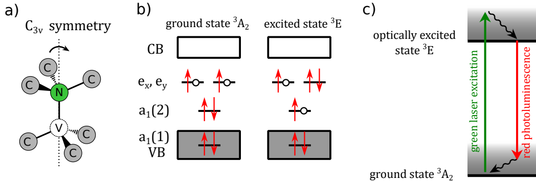
Figure 3.1: a) NV center embedded in a diamond crystal, with a C_{3v} symmetry around the NV axis. N : nitrogen, C : carbon, V : vacancy b) Detailed electronic structure of the NV^- center, the molecular orbitals are named after their symmetry. VB: Valance Band, CB: Conduction Band. c) Orbital ground and excited state of the NV^- center. Excitation is typically done at 532 nm in the phonon band (grey gradient) while the photoluminescence spectrum is mostly in the red, following phonon emission (wavy arrow).
