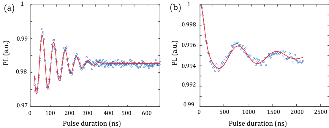
Figure 3.14: Rabi oscillations from NV centers in deposited diamonds for two different microwave powers in the presence of an externally applied magnetic field. All parameters are the same apart from the two microwave powers: a) \Omega_R = 16 MHz, b) \Omega_R = 1.3 MHz.
