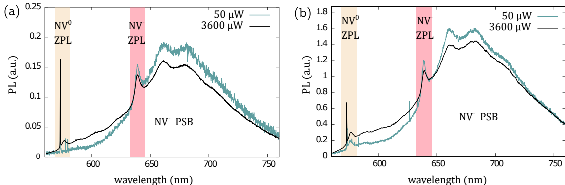
Figure 3.17: Optical spectras of NV centers embedded within a micro-diamond for two different powers for a) a levitating diamond and b) a diamond lying on a glass coverslip.
