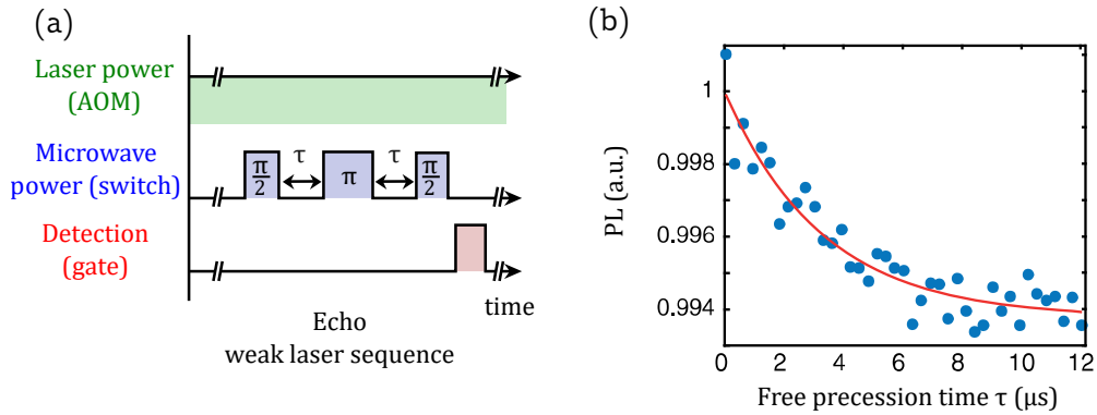
Figure 3.25: a) Echo sequence we use to measure the T_2^{echo} of the NV spins under weak laser. The axis break symbolises a long waiting time necessary to initialize the spins. b) PL as a function of the free precession time for an NV spin ensemble in a levitated micro-diamonds.
