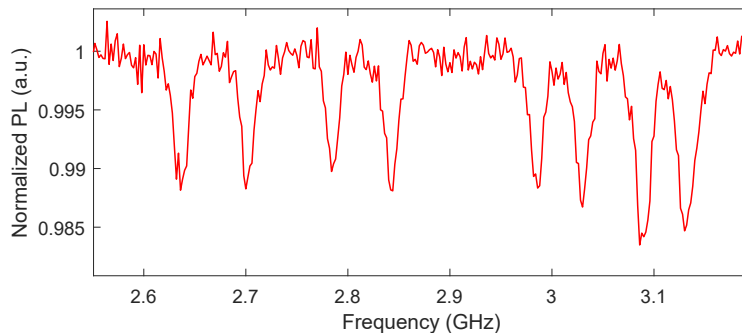
Figure 3.7: ESR spectrum for an NV centers ensemble within a single microdiamond taken under a magnetic field of about 100 G. We use a microwave power of 10 dBm.
