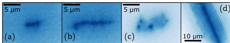
Figure 5.3: Image of a), b), c) a levitated micro-rod and d) a 15 \mu\text{m} wire taken for calibration of the magnification.
