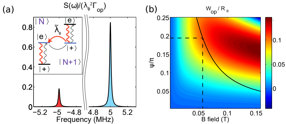
Figure 4.14: a) Power spectrum showing the emission ( \omega < 0 ) or absorption ( \omega > 0 ) of phonons under resonant conditions \omega_{e'} - \omega_+ = \omega_\phi . The inset shows the cooling mechanism as a cascade between the dressed states from rotational phonon numbers N + 1 to N . The parameters are: B = 2.6 mT, \Omega_R/(2\pi) = 0.5 MHz, \Delta/(2\pi) = 3 MHz and \Gamma_{\text{op}} = 10 kHz. b) Normalized cooling rate as a function of the B -field and \Psi/\pi for \Gamma_{\text{op}} = 100 kHz and \omega_\phi/(2\pi) = 5 MHz. The black line is the \psi parameter under resonant conditions as a function of the B -field for \Omega_R/(2\pi) = 1 GHz.
