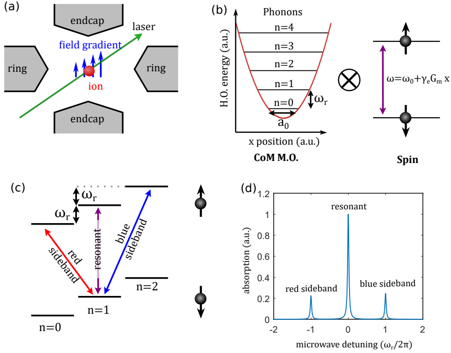
Figure 1.3: a) Ion trap: an oscillating voltage is applied between the ring and endcaps electrodes, resulting in harmonic confinement for ions at the center of the trap. A magnetic field gradient associated with a microwave field or a laser can be used to control the motion of the ion. b) Left: harmonic oscillator's potential energy (red curve) and the quantized phonon number states (black lines). a_0 is the amplitude of the zero-point fluctuations of the position. Right: two level system (spin one half) which energies depend on the position due to the field gradient and Zeeman effect. c) Dressed states for the two level system and a harmonic oscillator. The electronic transitions are addressed by a microwave transition, and cross-phonon transitions can occur due to spin-mechanical coupling. d) Absorption spectra of a trapped ion, the sidebands generated by the spin-mechanical coupling result in absorption (creation) of a phonon for the red (blue) sideband.
