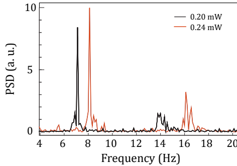
Figure 2.14: Power spectral density (PSD) of the back-scattered light from a levitated micro-diamond rotating due to radiation pressure.
