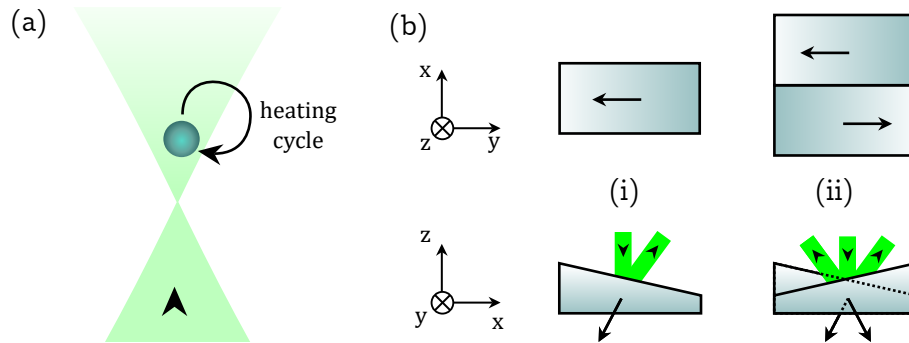
Figure 2.13: a) Example of heating mechanism for the center of mass of an isotropic particle. Here it follows a heating cycle in and out of the light beam, during which it gains energy from the radiation pressure. b) Effect of radiation pressure on basic shape: (i) prism-like particle, (ii) prisms of opposite slopes next to each other. Particles are shown from two point of view: the z optical axis (top) and the y axis. Black arrows indicate optical forces while light green beams show how the laser field is reflected off the particle.
