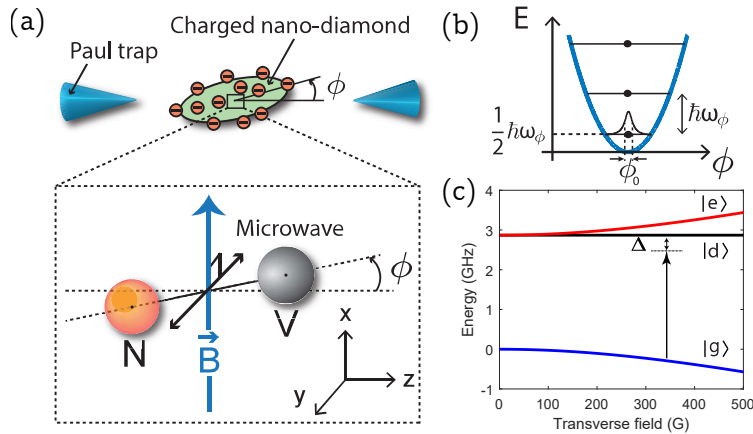
Figure 4.10: a) Scheme for spin-mechanical coupling between an NV spin and the librational mode of a Paul trap. b) Harmonic potential for \phi , with the energies of the first phonon Fock states and \phi_0 the amplitude of the zero-point fluctuations. c) Energies of the eigenstate of H_{NV} as a function of the intensity of the transverse magnetic field.
