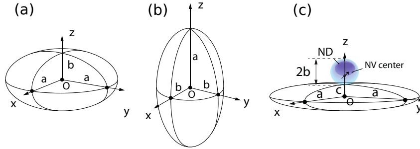
Figure 4.12: Proposed shapes for the levitating particles: a) Diamond oblate spheroid, b) Prolate spheroid and c) Composite particle made of a diamond sphere deposited on a thin disk, approximated by an oblate spheroid.
