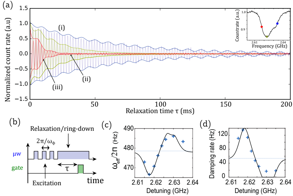
Figure 4.5: a) Ring-down of the librational modes of a levitating micro-diamond observed when a microwave is turned on (i) blue detuned, (ii) resonant and (iii) red-detuned from the magnetic resonance of a spins ensemble. Upper right caption: magnetic resonance mechanically detected, the three microwave frequencies (red, blue detuned and resonant) are marked by dots on the curve. b) Sequence we use for a ring down measurement. c) Frequency and d) damping rate of a librational mode during a ring-down as a function of the microwave detuning. Lines are simulation according to the model described in [77]
