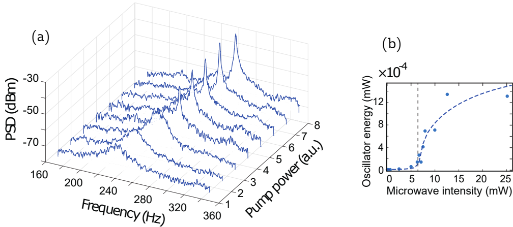
Figure 4.9: a) Evolution of the PSD with pump power of the blue detuned microwave. b) Threshold behavior of the oscillator’s energy as a function of the microwave power.
