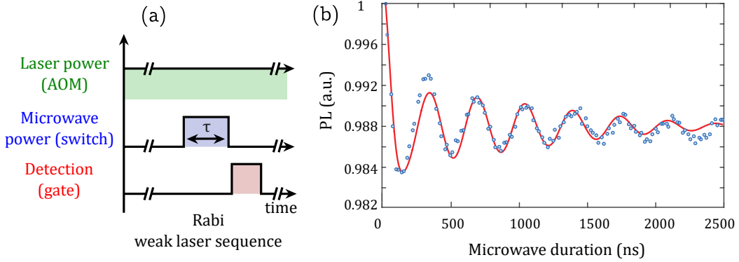
Figure 3.23: a) Shows the sequence that we apply given a weak laser excitation. The axis break symbolises a long waiting time necessary to initialize the spins (from a dozen to a hundred microseconds). b) Rabi oscillations from NV centers embedded in a levitated micro-diamond. We use 5 dBm of microwave power.
