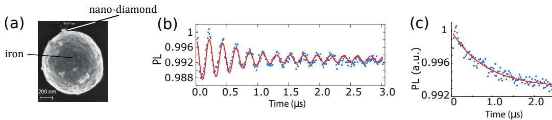
Figure 5.8: a) SEM image of a hybrid particle, with nano-diamond on the surface of an iron sphere. b) Rabi oscillations and b) Hahn echo from NV spins embedded in a nano-diamond lying on the surface of an iron sphere levitating in a Paul trap under atmospheric pressure.
