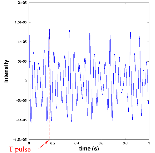
FIG. 5. Graph of the auto-correlation C_{T_{signal}, T_s}(\tau) of unit C : the maximum of correlation for T_{pulse} \simeq 0.17 s corresponds to a frequency f_{pulse} \simeq 6 Hz. The time T_{signal} is 4 s. (color online)
