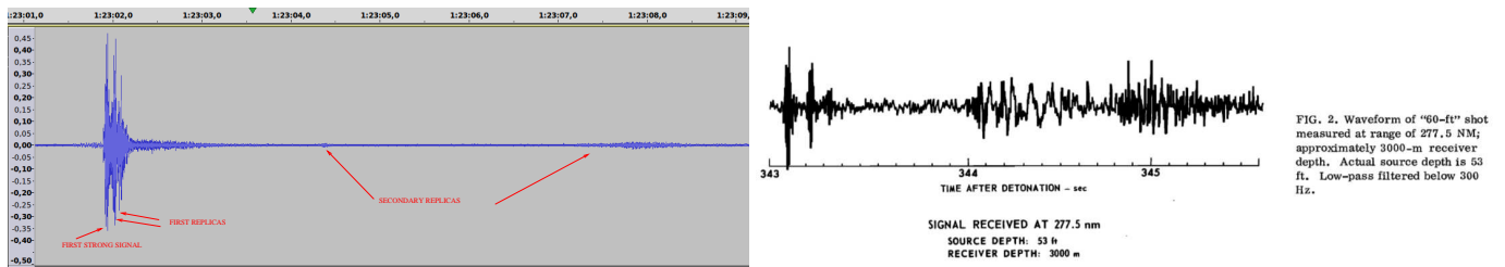
Figure 2: Explosion in wave form and its replicas (left) and a recording from [10] (right)
