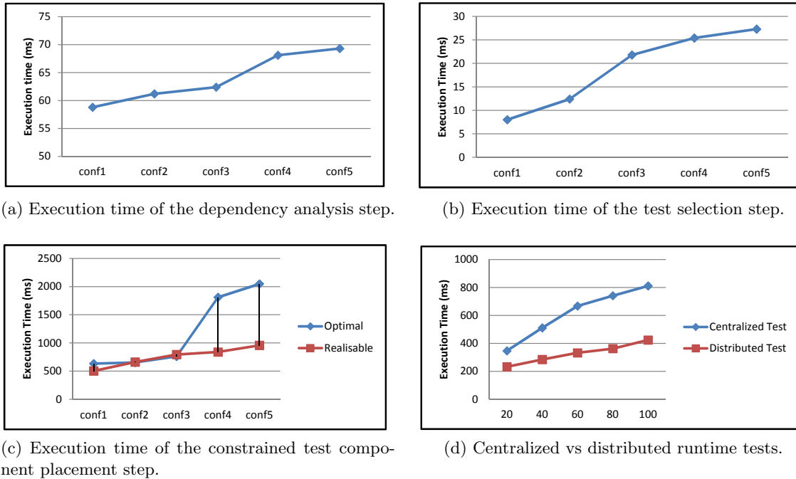
Figure 7.7: Execution time required by each step in the RTF4ADS framework.
