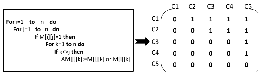
Figure 4.4: An adjacency matrix representing direct and indirect dependencies produced by the Roy-Warshall algorithm.
