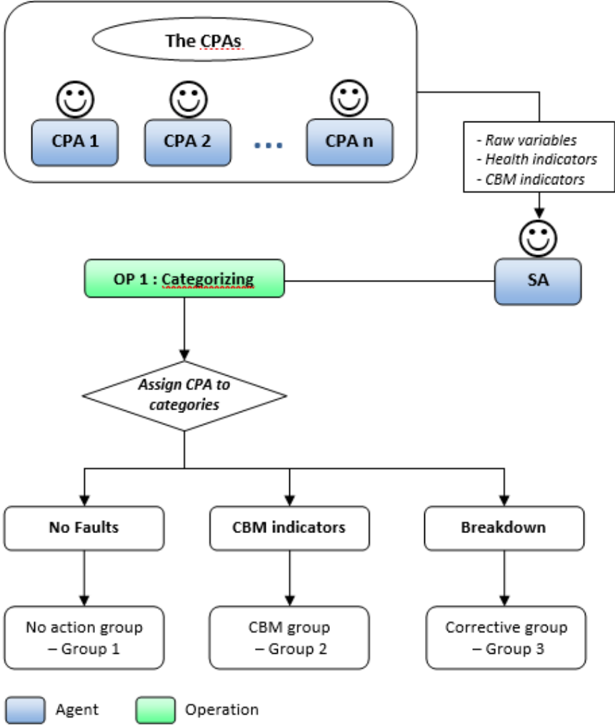
FIGURE III-3: CATEGORIZING PHASE
