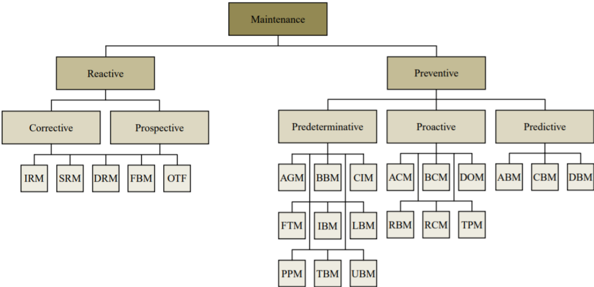
FIGURE I-9: MAINTENANCE TAXONOMY [107]
