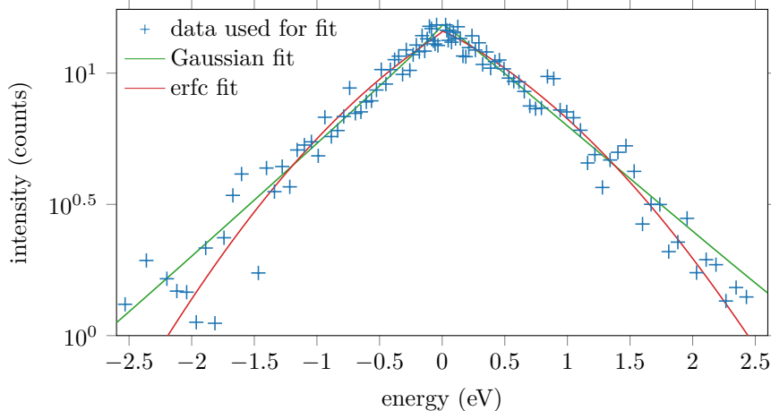
Figure 3.13: Representation of the logarithm of the Thomson scattering intensity as a function of the energy of the corresponding scattering electron (i.e., square of the spectral shift). The “+” symbols represent experimental data and the green and red lines correspond to the fitting functions for Gaussian and Druyvesteyn EVDFs, respectively.
