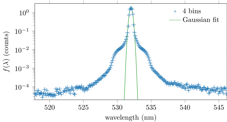
Figure 3.5: Instrument function profile for the THETIS diagnostic obtained using the 600 \text{ lines mm}^{-1} grating with a 300 \mu\text{m} spectrometer slit width. The “+” symbols in blue correspond to experimental data while the green line shows the Gaussian best fit of the profile.
