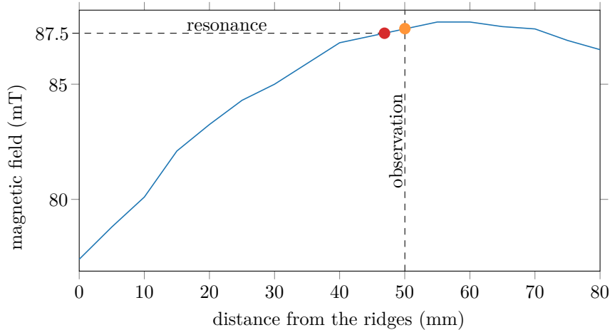
Figure 5.2: Axial profile of the magnetic field intensity along the axis of the plasma chamber for the configuration with (I_{B1}=64\text{ A}; U_{B1}=14.2\text{ V}) and (I_{B2}=68\text{ A}; U_{B2}=14.8\text{ V}) .
