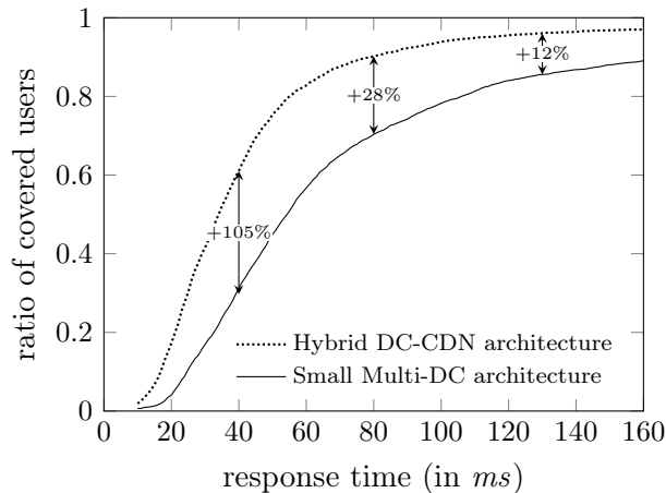
Figure 3.3 – Maximum achievable performances for an augmented infrastructure
