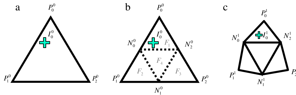
Fig. 7. (a) Step 1: determination of the face F containing I_0^0 . (b) Step 2: splitting the face F , inserting the new vertices: N_0^0, N_1^0, N_2^0 . (c) Step 3: image I_0^1 of I_0^0 in the next subdivision level.
