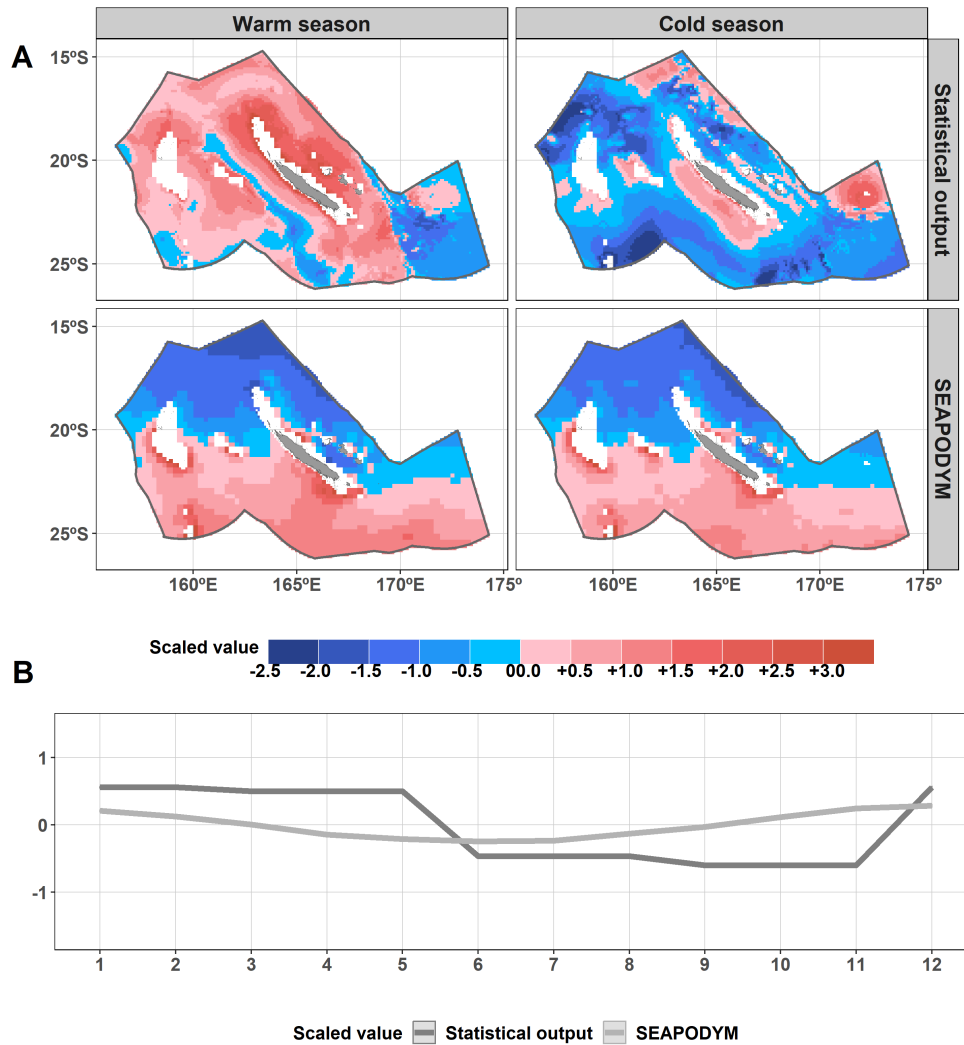
FIGURE 2.9 – Corrected backscatter values predicted on average for the hybrid GAMM2/SVM model with a variation coefficient inferior to 6% (Statistical output, Panel A, top row), and SEAPODYM-MTL model (panel A, bottom) averaged by season. Only cells predicted by SEAPODYM-MTL are shown in both rows of panel A. Same data averaged by month (panel B). Values on the three panels are scaled and centered for comparison.
