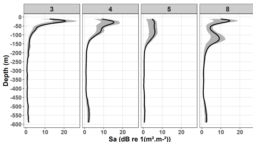
FIGURE 3.6 – Vertical profile means for each night acoustic class. The grey ribbon is the interquartile range.
