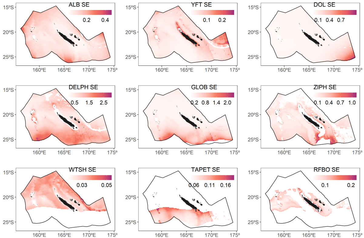
FIGURE 6.7 – Standard error (SE) predicted by the models (grey ribbons on Figure 2 and 3) for the nine spatial predictions in the same unit than for Figure 6.6.
