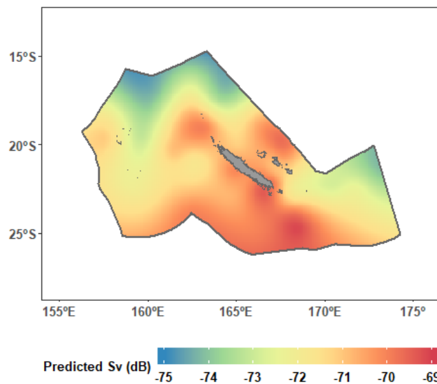
FIGURE 2.12 – Backscatter predicted by the GAMM1 by the spatial term (i.e. s(\text{lon}, \text{lat}) ).
