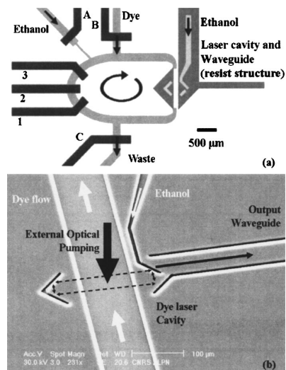
FIG. 1. (a) Schematic presentation of a tunable dye laser with a ring cavity and integrated microfluidic elements (The three adjacent control channels of the peristaltic pump are numbered 1, 2, and 3, whereas A, B, and C indicate the control channels of the fluid entrances and exit). (b) Scanning electron micrograph of the ring cavity made of SU-8 resist.
