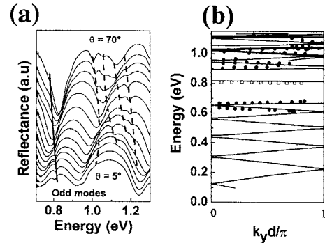
FIG. 5. Reflectance measurements along the \Gamma M orientation for the TE polarization on the PhC fabricated by soft UV-NIL and subsequent RIE. (a) The curves are vertically shifted for clarity. Curves from 5° to 70° with a 5° step are shown. Dashed curves indicate the position of the bulk mode resonances whereas the defect mode is indicated by a solid line. (b) Corresponding photonic bands folded into the reduced Brillouin zone due to supercell periodicity: experiments (empty squares for defect mode; filled circles for bulk modes) and theory (solid lines).
