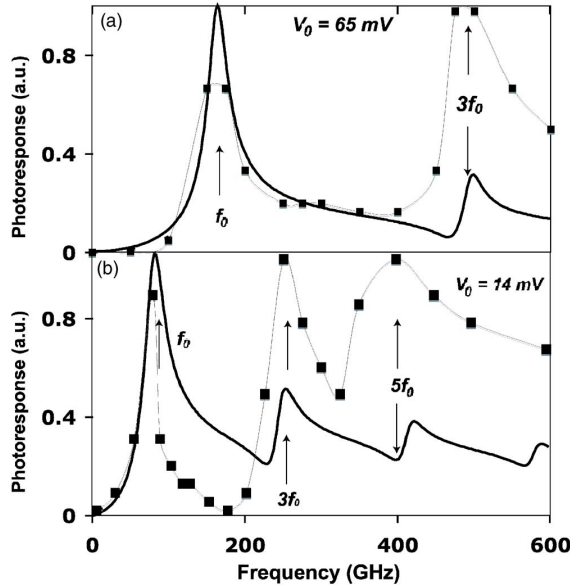
FIG. 2. (Color online) Photoconductive response vs excitation frequency ( 0 \text{ GHz} \leq \Delta f \leq 600 \text{ GHz} ) for (a) V_0=65 \text{ mV} and (b) V_0=14 \text{ mV} . Squares are experimental data joined by eye guidelines. Solid lines are calculation from Eq. (2). V_d=100 \text{ mV} to the source (ground). Arrows are for f_0 , 3f_0 , and 5f_0 .
