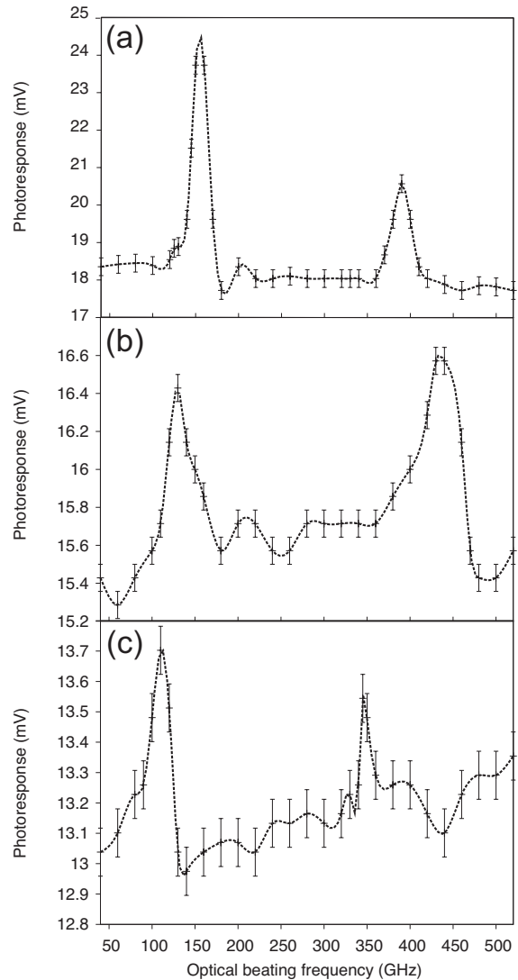
FIG. 16. Photoresponse vs optical beating frequency for a 400 nm gate-length transistor varying drain-source current and gate voltage. (a) V_d=750 mV ( I_d=1.5 mA) and V_0=170 mV. (b) V_d=600 mV ( I_d=870 \mu\text{A} ) V_0=120 mV. (c) V_d=550 mV ( I_d=520 \mu\text{A} ) and V_0=70 mV. Error bars are experimental data joined by eye guidelines.
