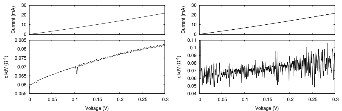
Figure 4.40 : Current-voltage characteristics and its derivative for a 5 \mu\text{m} long TLM structure maintained at 7 K (a) and 77 K (b).
