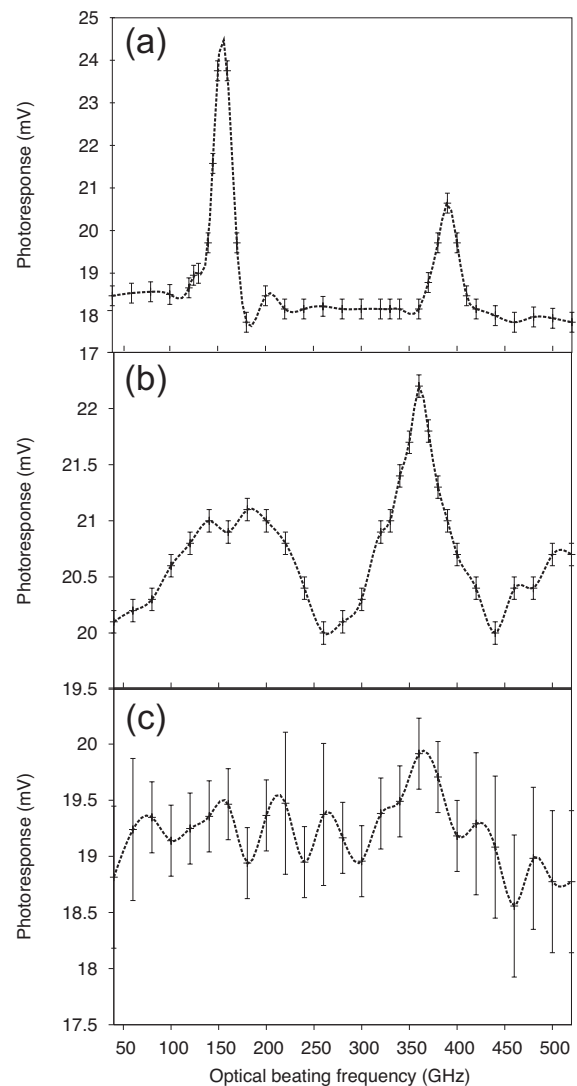
FIG. 10. Photoresponses as functions of the optical beating frequency and vs the applied drain-source current for a 400 nm gate-length transistor with V_0=170 mV. (a) V_d=750 mV ( I_d=1.5 mA), (b) V_d=500 mV ( I_d=1.3 mA), and (c) V_d=170 mV ( I_d=1 mA). Error bars are experimental data joined by eye guidelines.
