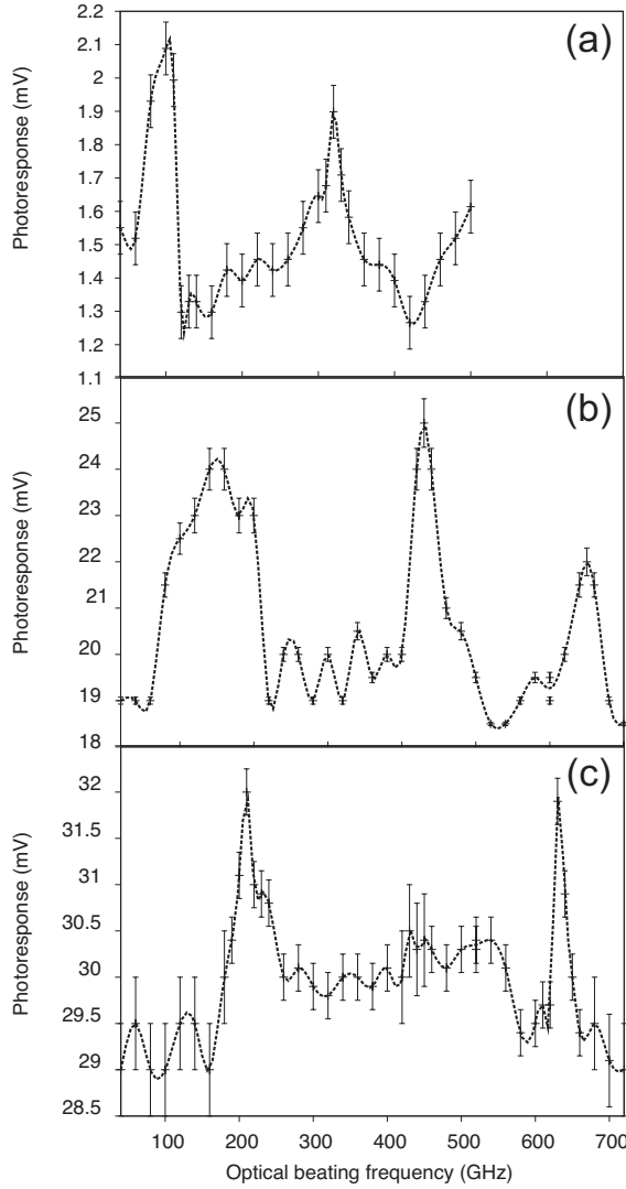
FIG. 4. Measured photoresponse vs the optical beating frequency for three gate-length transistors at fixed swing voltage V_0 \approx 170 mV and three biasing points. From (a) to (c): L_g=1500 nm: V_d=330 mV ( I_d=150 \mu A); L_g=400 nm: V_d=550 mV ( I_d=1.3 mA); L_g=200 nm: V_d=310 mV ( I_d=865 \mu A). Error bars are experimental data joined by eye guidelines.
