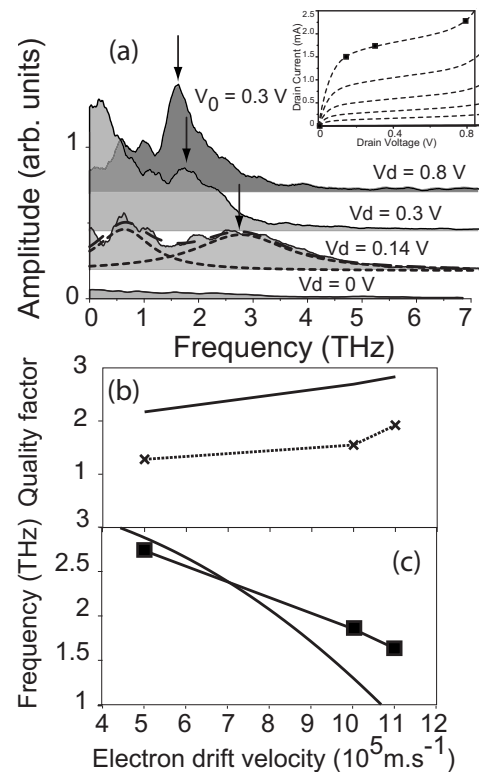
FIG. 3. (a) Emission spectra by varying the drain voltage from 0 up to 0.8 V. The dashed and dotted lines are Lorentzian fits of curve at V_0 = 0.3 V and V_d = 0.14 V. Inset: static output characteristics for a gate potential varying from -0.2 to 0 V with a 0.05 V step under illumination. (b) Quality factor and (c) peak frequency variation as a function of the average electron drift velocity.
