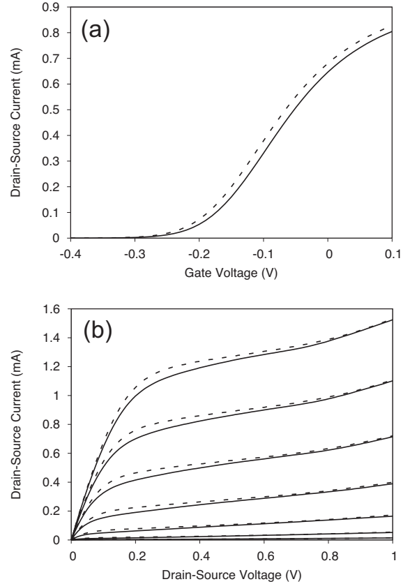
FIG. 3. HEMT transfer and output characteristics for a HEMT with gate-length L_g=200 nm. (a) I_d vs V_g at V_d=100 mV. Dark dc drain-current (solid line) and under illumination (dashed line). (b) I_d vs V_d varying V_g from 0 down to -300 mV with -50 mV steps. Dark dc drain-current (solid line) and under illumination (dashed line).
