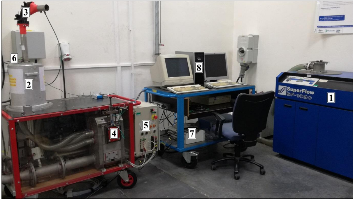
Figure II-3 – Dynamic Flow Bench
