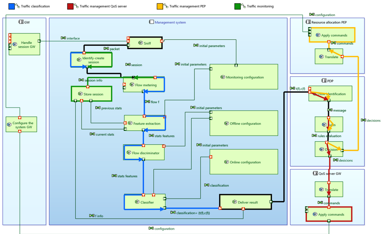
Figure 3.13: System architecture.
