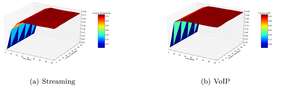
Figure C.2: F-score of the dynamic ensemble varying the number of base classifiers and the maximum depth of the DTs
