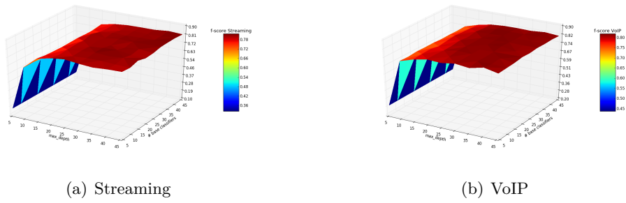
Figure C.6: F-score of the dynamic ensemble varying the number of base classifiers and the maximum depth of the DTs
