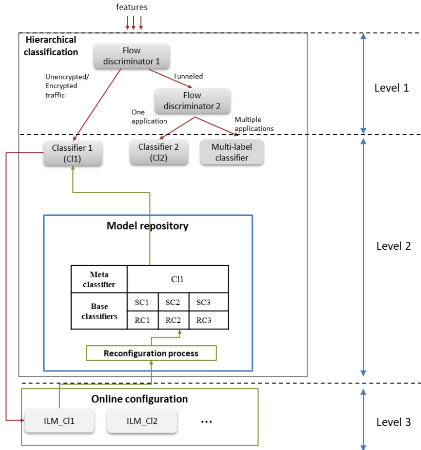
Figure 6.1: Hierarchical classification system.
