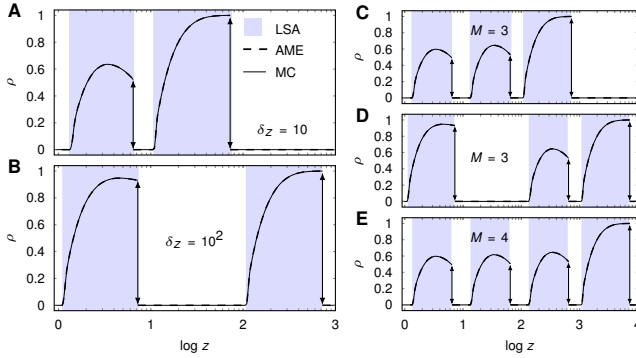
Figure 4.7 – Steady state global cascade size as a function of average degree z , for constant threshold \phi = 0.15 and maximal weight heterogeneity ( \delta_w = 10^{-6} ), using the weighted sum rule. Degree distributions are Poisson and overlap is \gamma = 0 . Shaded intervals due to LSA indicate systems with a positive leading eigenvalue (see Chapter 2); dashed lines indicate the steady state solution of Eqn. 4.9; and MC solutions are given by the solid curve (error bars narrower than line width). (a, b) Increasing density skewness \delta_z delays the onset of high- z phases of contagion, and allows larger cascades in low- z phases in an M = 2 layer multiplex. (c-e) Increasing the number of layers to M = 3 and 4 induces 6 and 8 phase transitions in cascade size, respectively. (d) Varying \delta_z , such that z_2/z_1 = 100 , and z_3/z_2 = 10 . MC results are averaged over 10^3 realizations of single node perturbation, with N = 10^7 .
