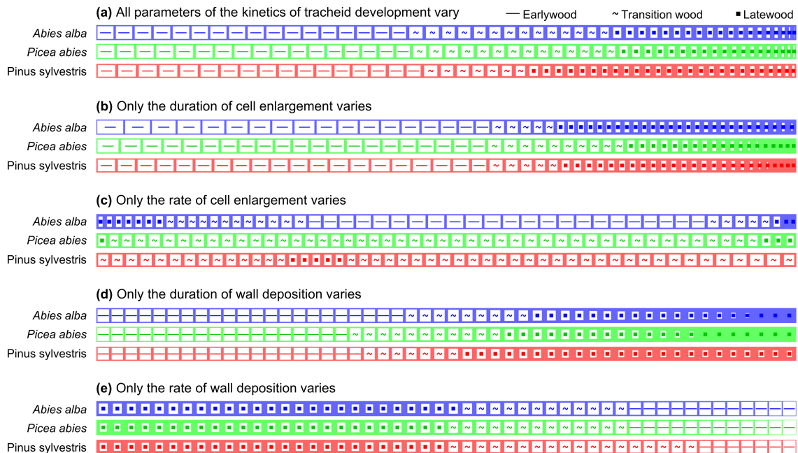
53 — Figure 6.7 | Schemes of the different tree rings formed when the different parameters of the kinetics of tracheid development are changed one at a time. Figure from Cuny et al. {2014}.
