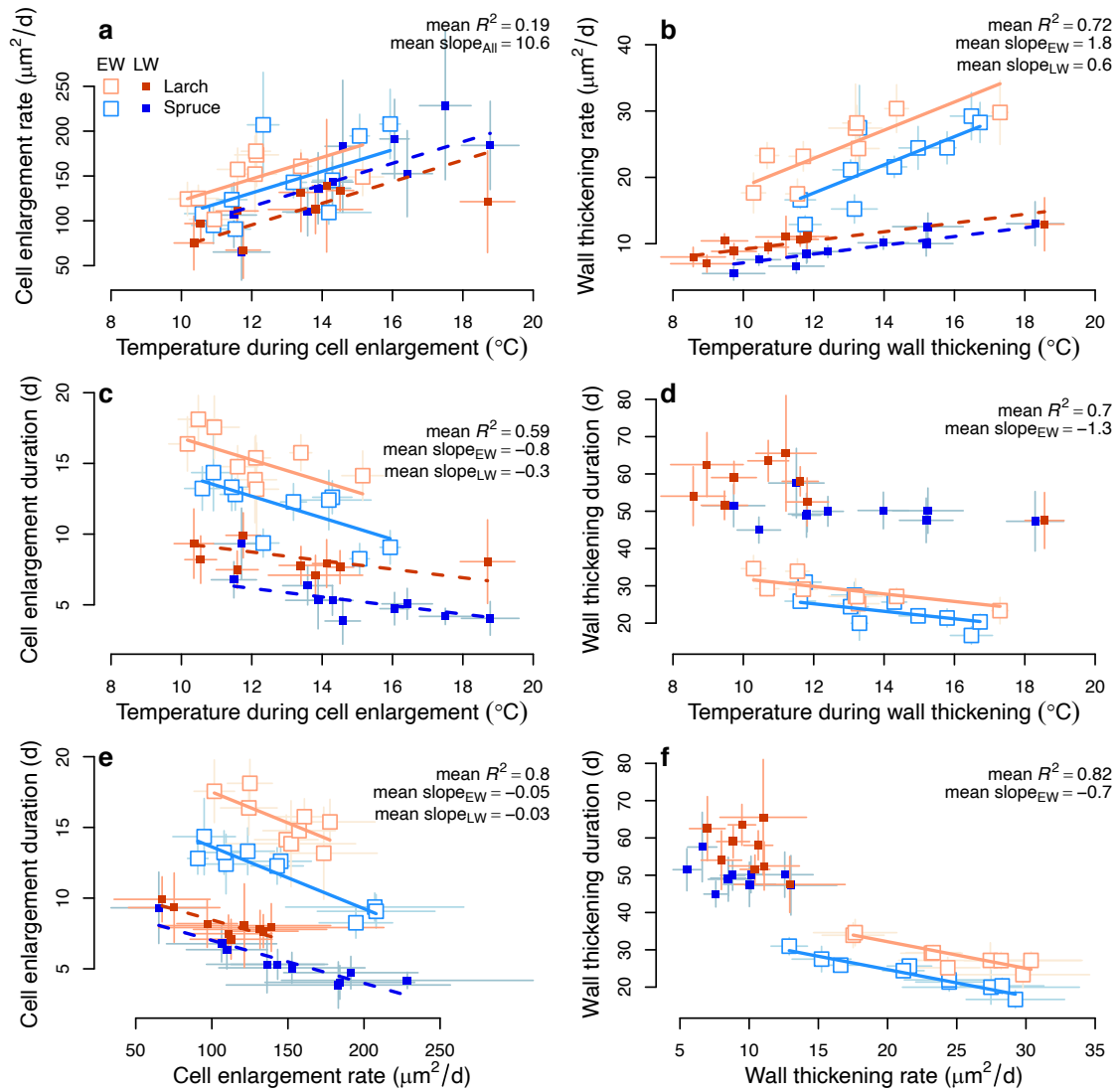
59 — Figure 6.13 | Influence of air temperature on xylem cell dimensions along the Donon-Lötschental gradient.
