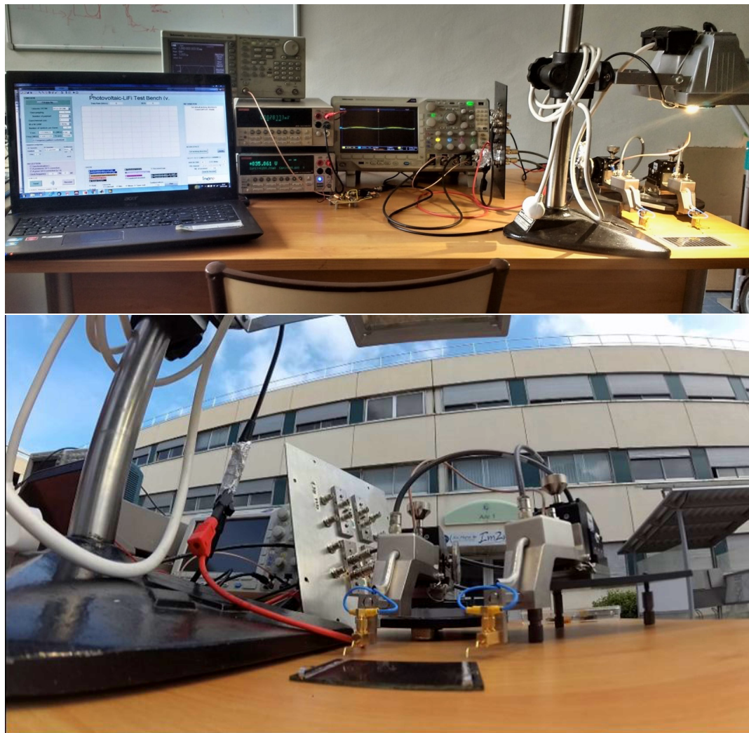
Figure 8.26 – Photo du banc en configuration outdoor
