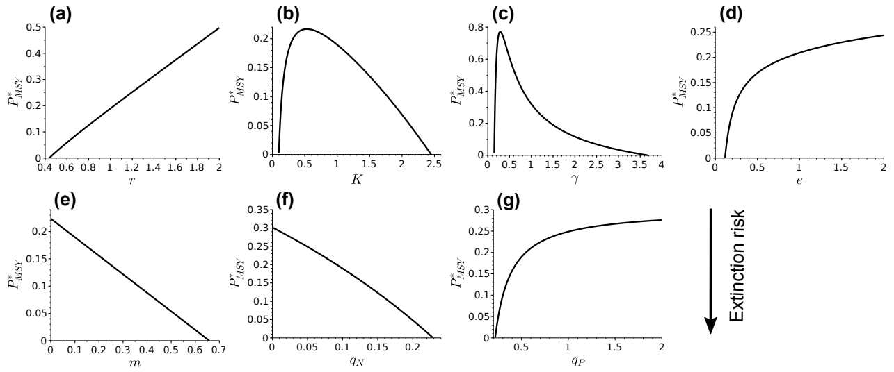
Figure A1: Sensitivity of predator equilibrium density at MSY to parameter values. For each value of the considered parameter, the predator equilibrium density is computed while the other parameters are kept constant. The extinction risk of the predator increases with decreasing predator densities. (a) Varying prey growth rate r . (b) Varying prey carrying capacity K . (c) Varying predator attack rate \gamma . (d) Varying predator conversion efficiency e . (e) Varying predator mortality rate m . (f) Varying prey catchability q_N . (g) Varying predator catchability q_P . Constant values of the parameters are: r = 1 , K = 1 , m = 0.1 , e = 0.7 , \gamma = 1.5 , q_N = 0.1 , q_P = 0.5 .
