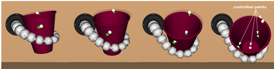
Figure 5.12: Simulation of a soft gripper holding a deformable cup subject to gravity. Here we optimize the cables displacements to control the position/orientation of the cup. A phantom of the cup target is shown in transparency. The cup have four controlled points represented by the green spheres. The corresponding targets are represented by the white spheres.
