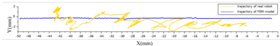
Figure 4.18: 2D trajectory of the real cable-driven soft robot end-effector, with corresponding trajectory of the FEM model. 3D average error of 3.6mm.
