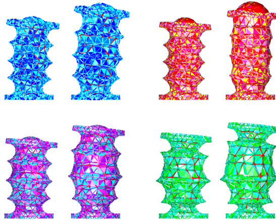
Figure 3.9: Difference between co-rotational (blue), Mooney-Rivlin (green), Saint-Venant Kirchhoff (red) and Neo-Hookean (purple) models on the accordion example. The results of each model are superposed. Imposing the same volume growth.
