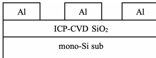
Fig. 38. Cross-sectional schematic of ICP-CVD \text{SiO}_2 MOS capacitor.
