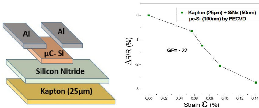
Figure 3.18: GF determination for Kapton (25 \mu\text{m} ) + SiN x (50 nm) + N-type \mu\text{C-Si} (100nm).
