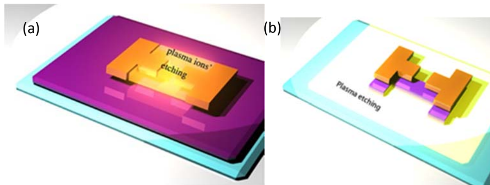
Figure 2.5 Schematic of the RIE plasma etching for the channel's definition (a) and device's isolation (b).
