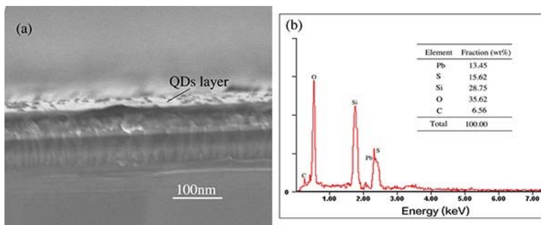
Figure 3.8 (a) The cross-sectional SEM image of spin-coated QDs layer in the oxidized silicon wafer. (b) Compound measurements of the PbS QDs through attached EDS spectrum in the SEM.
