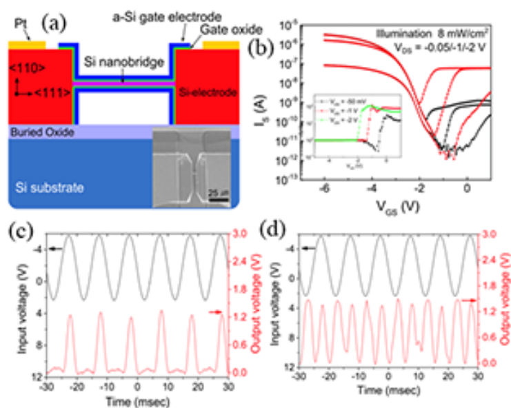
Figure 1.13 (a) The silicon nanobridge TFT's device structure. (b) The transfer IV characteristic of this TFT under illumination. The output signal without (c) and with (d) light [64].
