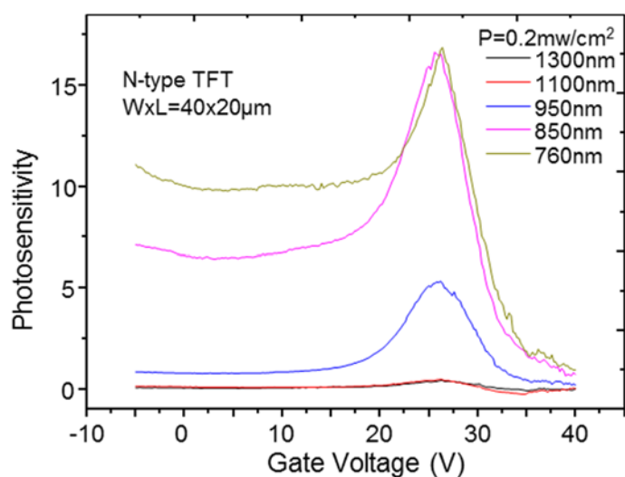
Figure 4.11 Photocurrent ( (I_{\text{Light}} - I_{\text{Dark}})/I_{\text{Dark}} ) of N-type to 0.2 \text{ mW/cm}^2 power light at different IR wavelength.
