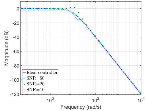
(b) Obtained closed-loops with controllers identified through the subspace approach under LMI constraints and using frequency-weighting.
