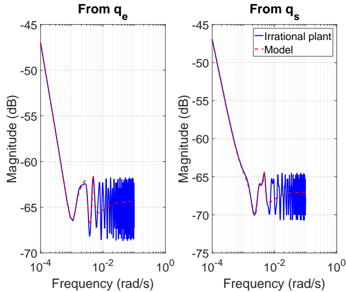
Figure 8.13: System dynamic for nominal flow Q_0 = 1400 \text{ m}^3 \cdot \text{s}^{-1} : original plant in solid blue and approximation obtained in [Dalmas et al., 2016] in dashed red.
