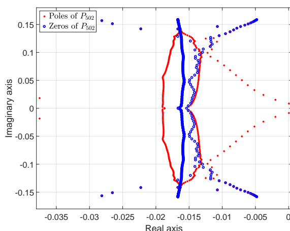
Figure 8.2: Poles and zeros of the rational model \mathbf{P}_{502}
