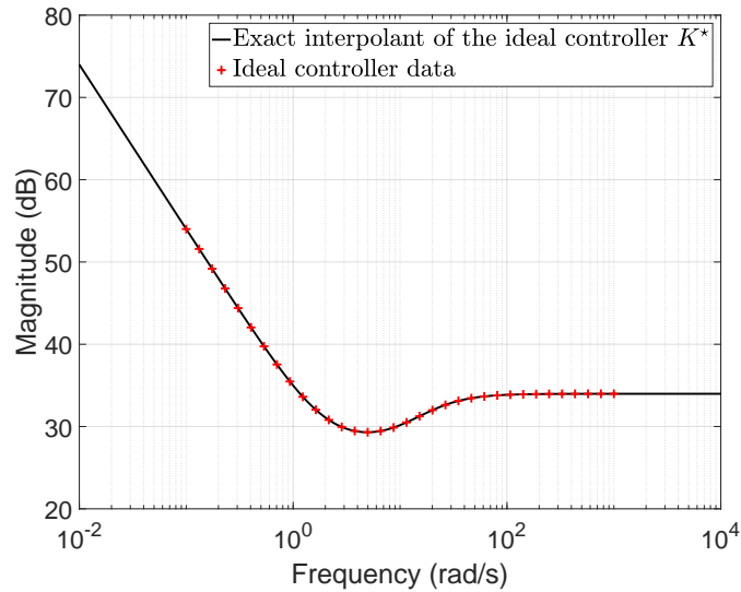
Figure 4.2: Interpolation of the ideal controller for the DC motor example.
