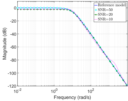
(a) Obtained closed-loops with controllers identified through the enhanced Loewner framework.
