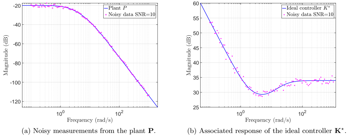
Figure 5.1: Use of noisy frequency-domain measurements from the DC motor (SNR=10) and computation of the frequency-response of the associated ideal controller \mathbf{K}^* .
