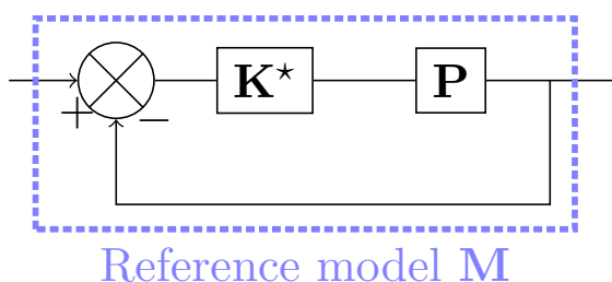
Figure 6.1: The ideal case: feedback interconnection obtained with the ideal controller.
