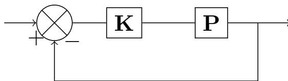
Figure 7.1: The resulting closed-loop: \mathbf{K} is a reduced-order model of the ideal controller \mathbf{K}^* .
