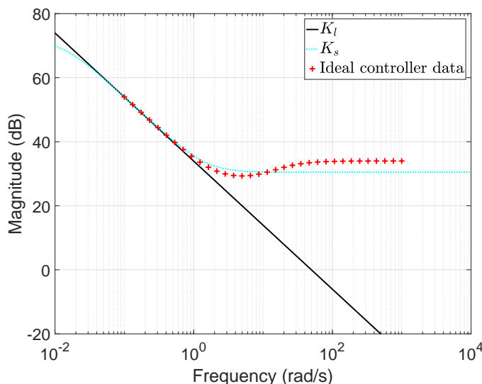
Figure 4.4: Identification of the first-order controllers \mathbf{K}_1 and \mathbf{K}_s , respectively through the Loewner framework and the subspace approach.
