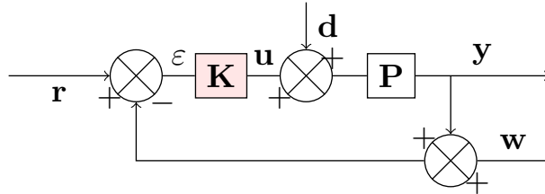
Figure 2.1: Considered feedback structure.
