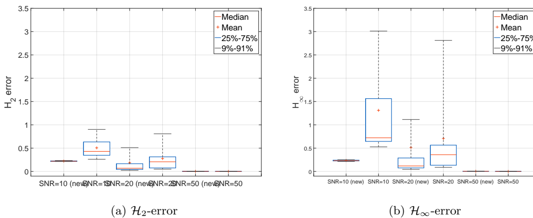
Figure 5.9: Impact of the noise on the performances obtained with the controllers identified through the subspace approach.
