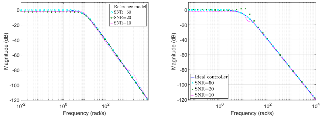
(a) Obtained closed-loops with controllers identified through the enhanced Loewner framework.
