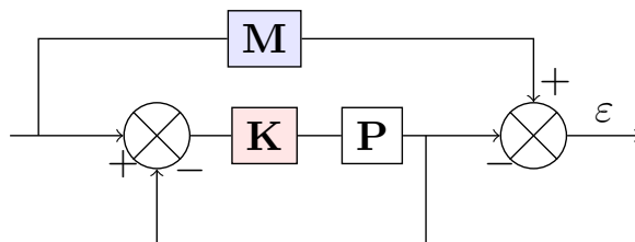
Figure 9.1: Problem formulation: \mathbf{M} is the desired closed-loop, \mathbf{P} is the plant and \mathbf{K} the controller to be designed.
