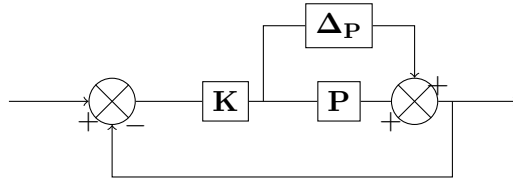
Figure 7.13: Stability robustness analysis scheme.
