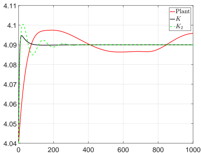
Figure 8.9: Simulation of the passage to a new steady state for the closed-loops built with the second-order controller \mathbf{K}_2 obtained by the proposed algorithm and \mathbf{K} , the one obtained in [Apkarian and Noll, 2018].
