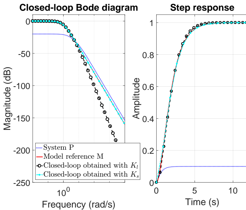
Figure 4.7: Closed-loop performances achieved in the DC motor example with first-order controllers designed using a reference model \mathbf{M} defined as in (4.6) with \omega_0 = 1 \text{ rad}\cdot\text{s}^{-1} and \xi = 1 .
