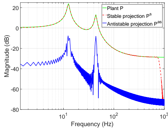
Figure 6.4: Projection of \{\omega_i, P(i\omega_i)\}_{i=1}^N to detect the presence of unstable poles.
