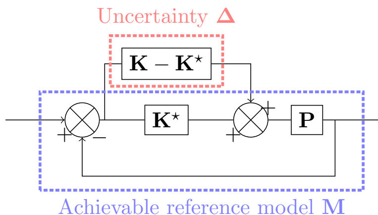
Figure 7.2: Stability analysis scheme: the controller modelling error is written as an uncertainty.
