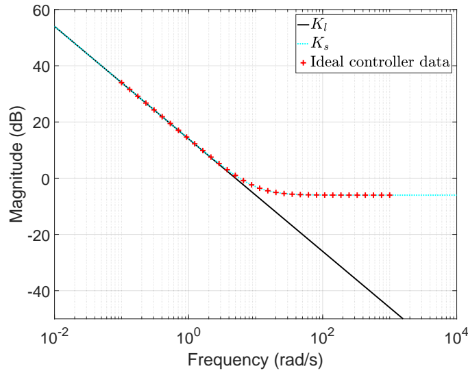
Figure 4.6: Identification of first-order controllers through the Loewner framework and the subspace approach for the DC motor for a reference model defined as in (4.6) with \omega_0 = 1 \text{ rad}\cdot\text{s}^{-1} and \xi = 1 .
