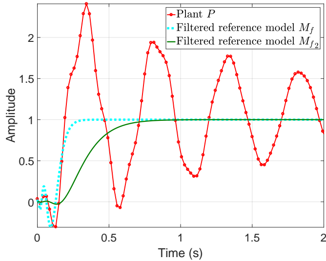
Figure 6.9: Step response of the filtered reference models \mathbf{M}_f and \mathbf{M}_{f_2} , and of the plant \mathbf{P} : the estimation of the instabilities should be used to modify the performance specifications if necessary.
