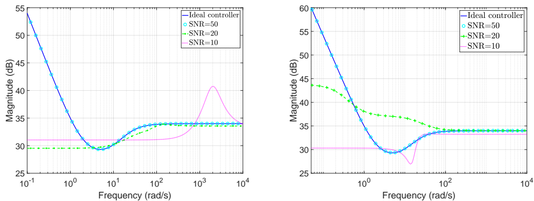
(a) Through the Loewner framework combined with the \mathcal{RH}_\infty -projection and the residue-based reduction. (b) Through the subspace approach under LMI constraints and using a frequency-weighting.
