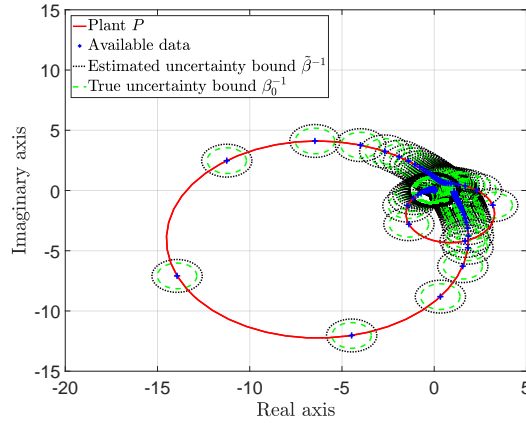
Figure 7.16: Robust stability analysis on the flexible transmission benchmark: the circles represent the plant's behaviours \tilde{\mathbf{P}} such that the plant's uncertainty \Delta satisfy (7.8).
