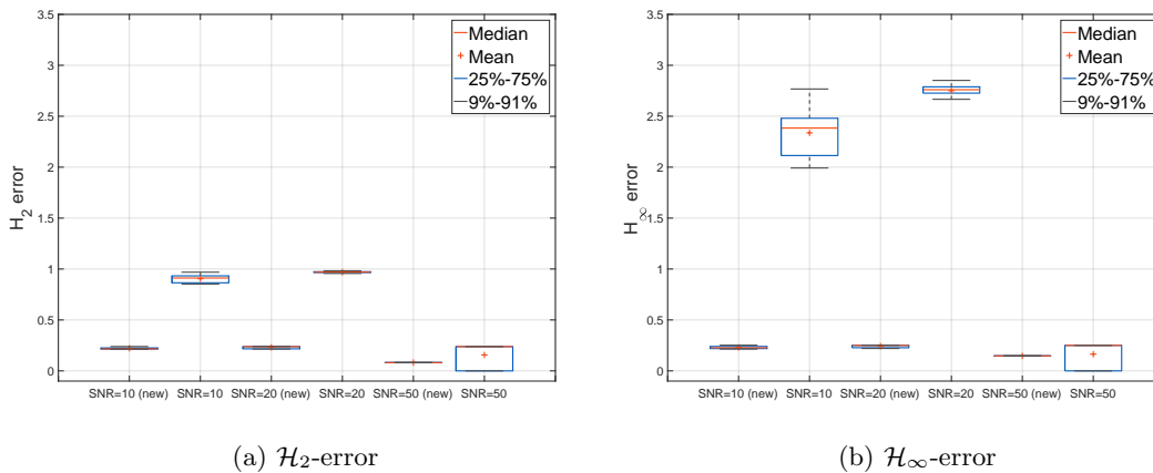
Figure 5.8: Impact of the noise on the performances obtained with the controllers identified through the Loewner framework.
