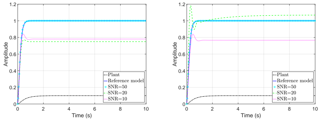
(c) Step responses obtained with controllers identified through the enhanced Loewner framework.
