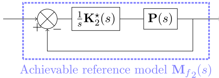
Figure 7.11: Enforcing the presence of an integrator in the controller through the proposed method in the DC motor example.
