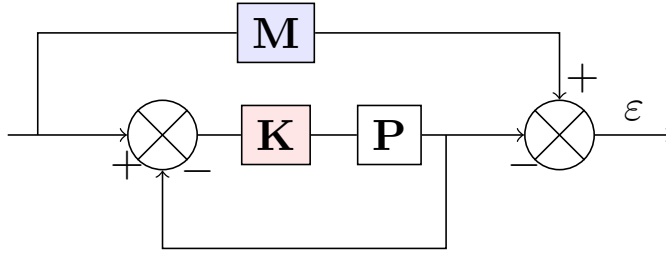
Figure 4.1: Problem formulation: \mathbf{M} is the desired closed-loop, \mathbf{P} is the plant and \mathbf{K} the controller to be designed.
