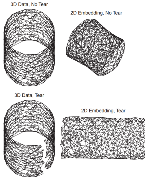
FIGURE 4.4: Like for the torus, Isomap fails to embed a 3D cylinder in a 2D space while preserving its similarity graph (upper panels). However, DR is successful if the cylinder has been preemptively "cut" (lower panels). From van der Maaten et al. (2008)
