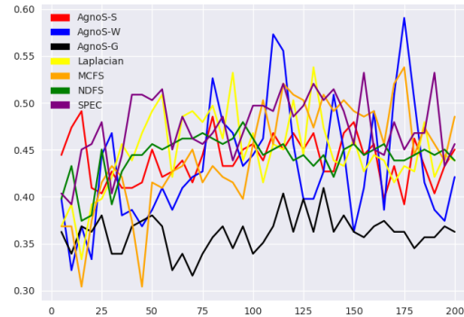
FIGURE 6.4: ACC score w.r.t. selection subset size k , on TOX171
