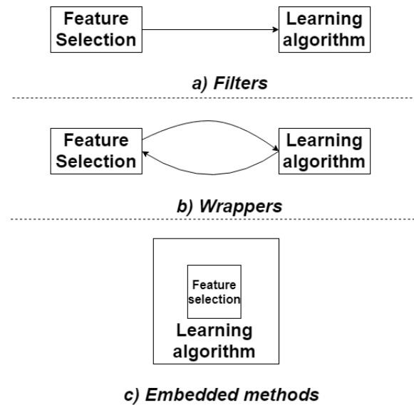
FIGURE 3.17: Schematic of filters, wrappers and embedded methods.
