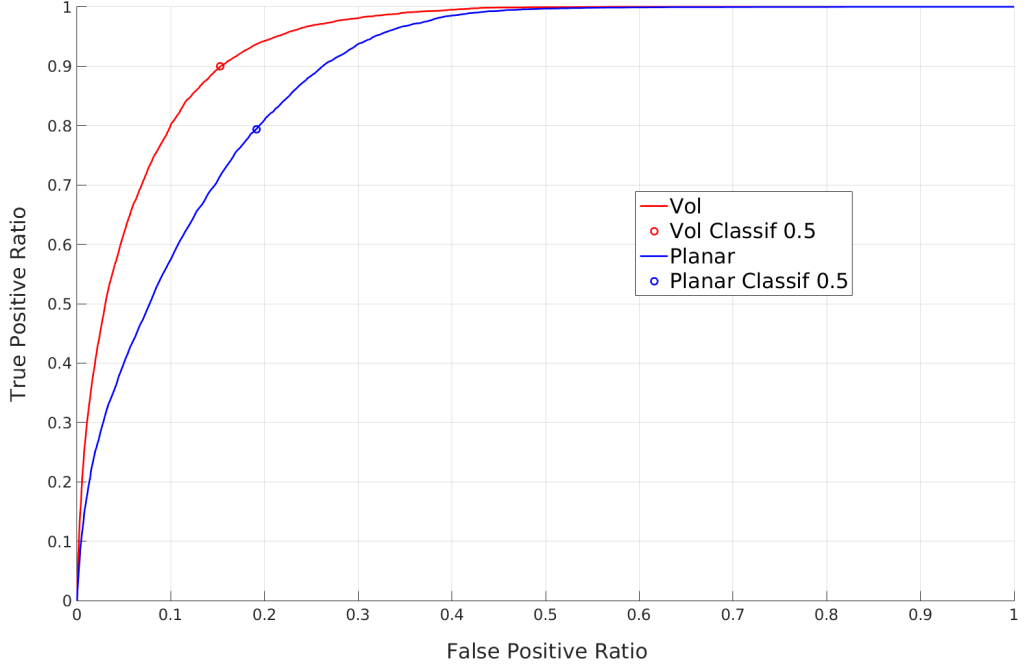
Figure 3.6: ROC Curves of two different classifiers using planar and volumetric receptive fields, on the sparse synthetic data. Circles represent thresholds that optimize sensitivity + specificity.
