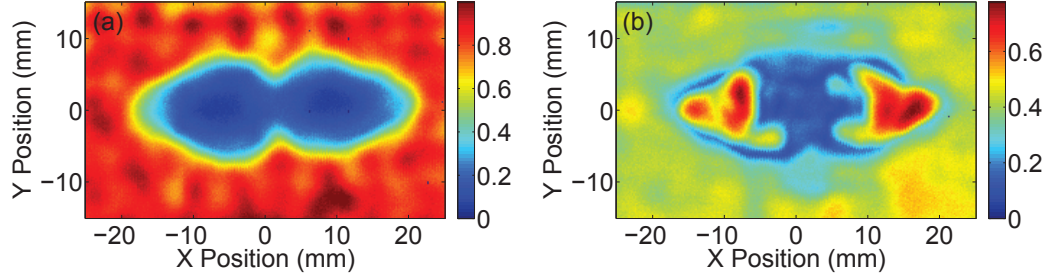
Figure 3.21: Ultrasonic C-scan results (a) in transmission and (b) in reflection modes. The ultrasonic waves are incident from the top surface of the sample. The contrast is based on the absolute value of the amplitude of the second-round signal in transmission and the second echo in reflection.
