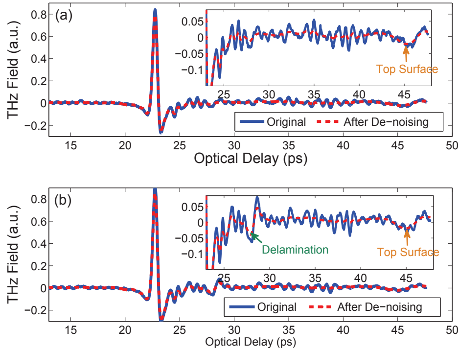
Figure 3.14: Typical reflected THz waveforms with and without wavelet de-noising in the region (a) without and (b) with delamination.
