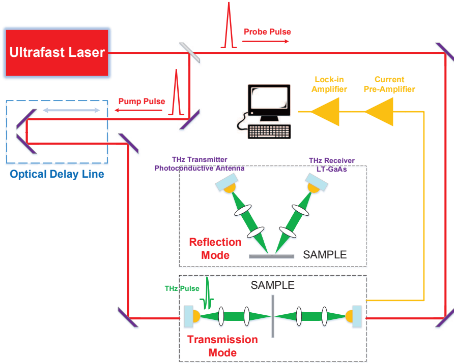
Figure 2.1: Schematic diagram of THz time-domain spectroscopy (TDS) system in both reflection and transmission configurations.
