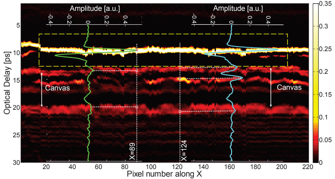
Figure 5.15: The THz B-scan based on the raw signal with the cross-section Y = 150 . Two typical THz reflected signals are plotted corresponding to the THz B-scan, with the waveform at pixel (89, 150) in green and the waveform at pixel (124, 150) in blue.
