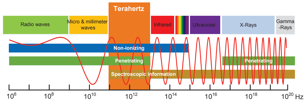
Figure 1.1: The terahertz portion of the electromagnetic spectrum.
