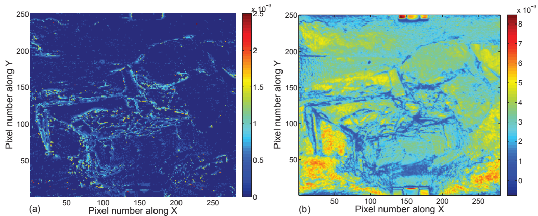
Figure 5.7: THz C-scans based on the Type I signal and the main peak indicating the surface feature of the painting.
