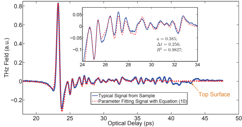
Figure 3.13: Multiple parameter regression analysis of measured THz waveform without delamination to identify the water-vapor effect.
