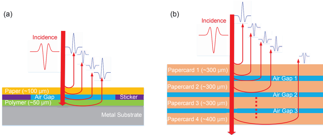
Figure 4.11: Two samples with multi-layered structures. (a) Sample A: a three-layered structure, which is composed of one copy paper, air gap and one polymer coating; (b) Sample B: a seven-layered structure, which is composed of four different papercards with air gaps between them.
