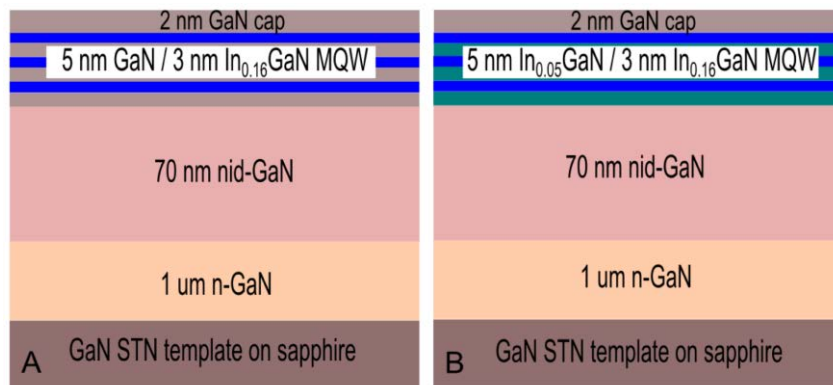
Figure 52 : Structure schematic of MQW sample A with GaN barrier and sample B with In 0.05 Ga 0.95 N barrier.
