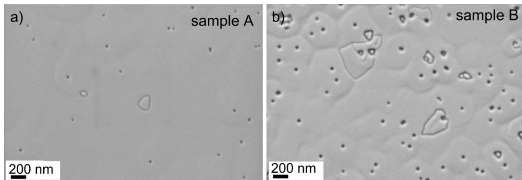
Figure 53 : SEM surface morphology of MQW sample A with GaN barrier (a) and sample B with In 0.05 Ga 0.95 N barrier (b).
