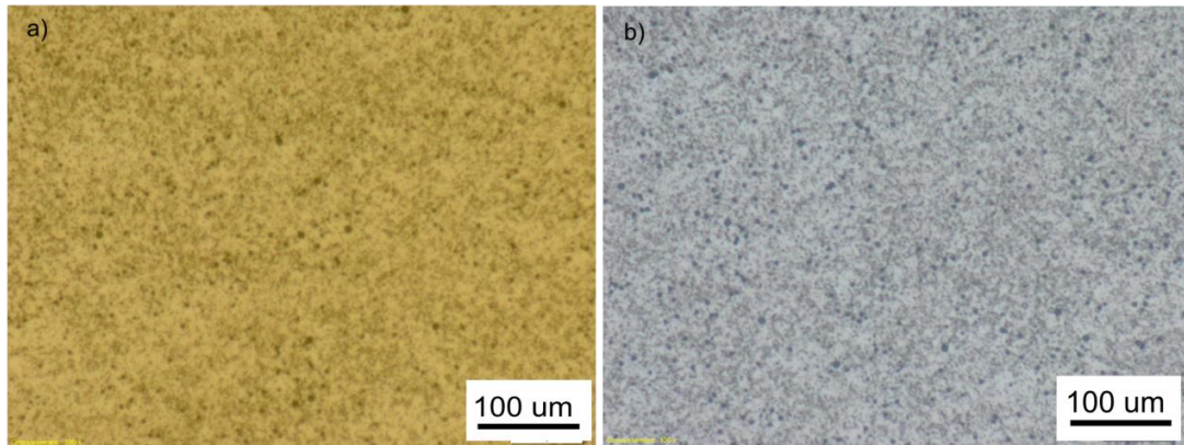
Figure 84: The LED wafer surface before (a) and after (b) HCl cleaning.
