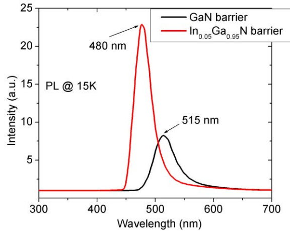
Figure 56 : Low temperature photoluminescence of 25% In-content MQW sample with GaN barrier and with \text{In}_{0.05}\text{Ga}_{0.95}\text{N} barrier.
