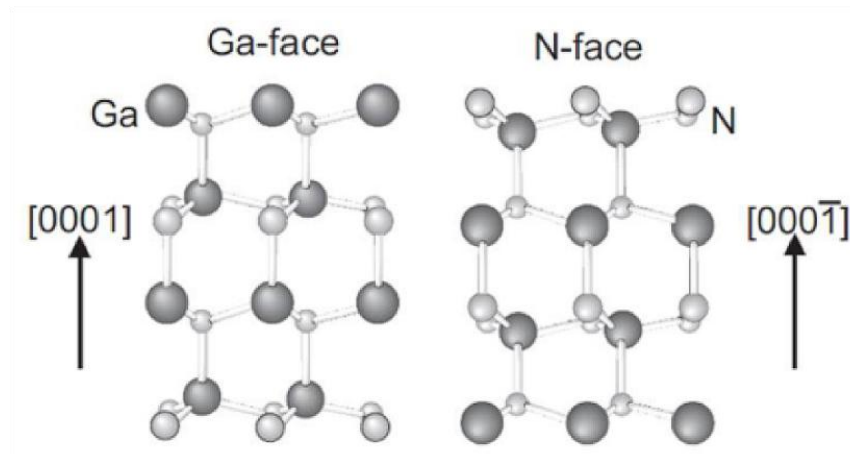
Figure 7: The two different faces of GaN: Ga-polar and N-polar [50].
