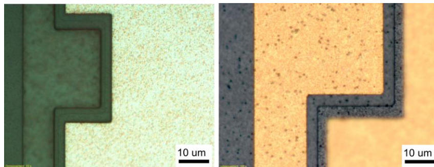
Figure 91: n-contact after lithography, metal deposition, lift-off (left), and then the resist was removed and annealed (right).
