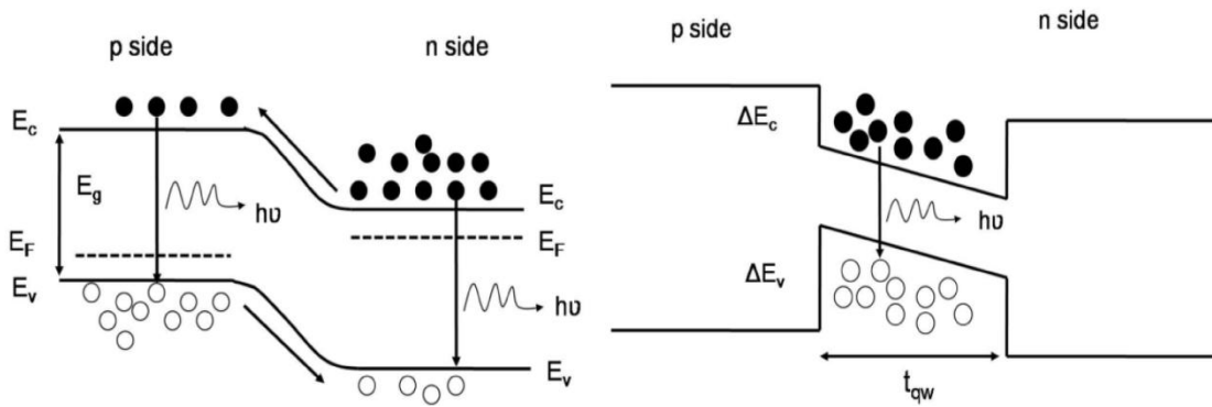
Figure 14: Homo-junction and hetero-junction LEDs (schematically).
