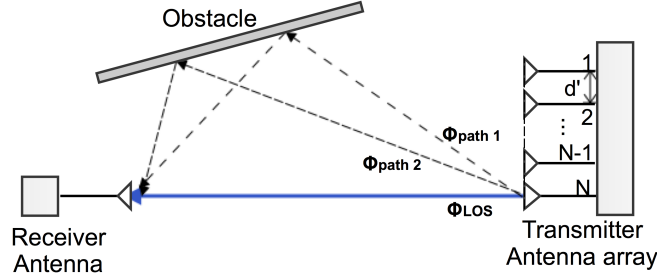
FIGURE 2.4: Signal radiation from an N -element uniform linear antenna array: The k -th antenna transmits a signal with a phase shift of e^{-j2\pi(k-1)\frac{d'}{\lambda}\sin(\phi)} relative to the reference antenna.
