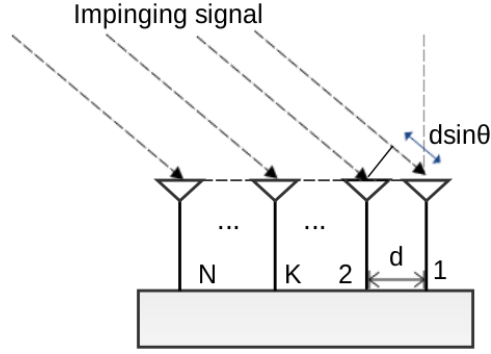
FIGURE 3.8: Signal impinging on an N -element uniform linear antenna array: Each antenna receives a copy of the signal with a phase shift k.d.\sin(\theta) relative to the reference element (First antenna), with d , the antenna spacing, in the order of half a wavelength.
