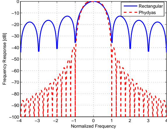
Fig. 2. OFDM (referred as "rectangular") and FBMC (referred as "Phydyas") Power Spectral Densities
