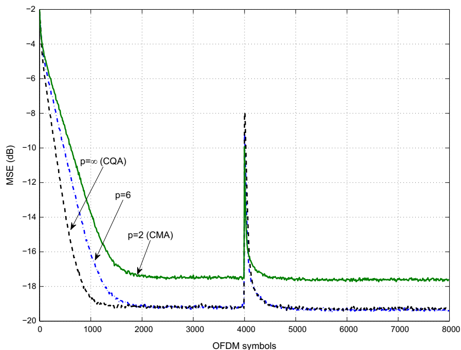
Fig. 12. Tracking performance of CMA, CNA-6, and CQA with PAP using DR2.
