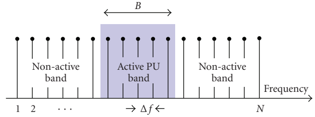
FIGURE 13: Frequency distribution with one active PU band.
