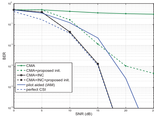
Fig. 6: BER versus SNR of the proposed equalizer compared to [1].
