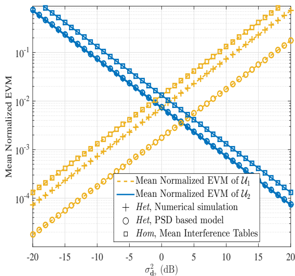
Figure 3.23: Mean Normalized EVM of users \mathcal{U}_1 and \mathcal{U}_2 in the scenarios Het and Hom
