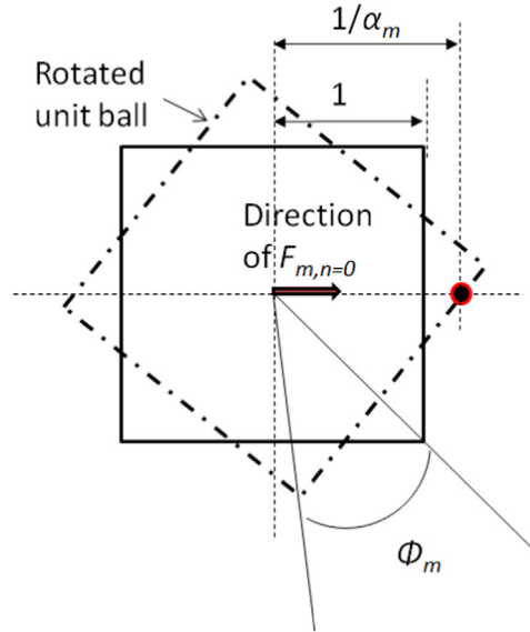
Fig. 4. Geometrical interpretation of the effect of the phase rotation \phi_m on \alpha_m , using p = \infty .
