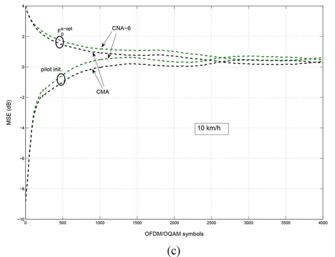
Fig. 10. MSE performance of CNA-6, CNA-2 (CMA) versus OFDM/OQAM symbols using the initialization F_{m,0}^{s-opt} compared with the initialization using a preamble, for three receiver speeds: (a) 1 km/h, (b) 3 km/h, and (c) 10 km/h.
