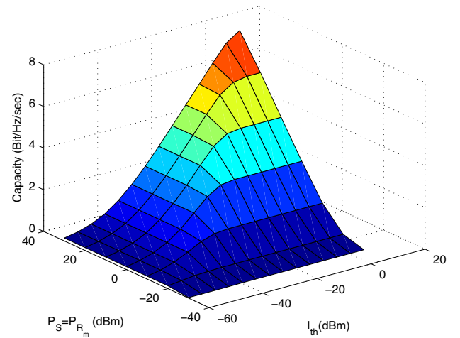
Fig. 3. Achieved capacity vs allowed interference thresholds and power budget constraints.
