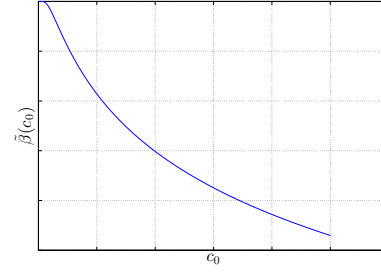
Figure 3: Curve of the function \tilde{\beta}(c_0) .
