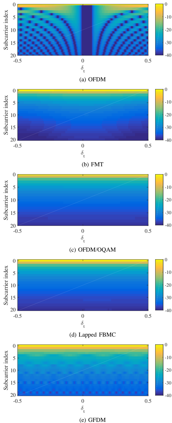
Fig. 4: Interference in dB caused by an active D2D at subcarrier 0 on 20 neighboring OFDM subcarriers of the incumbent in function of \delta_t for different waveforms. Only OFDM shows a figure significantly varying along the \delta_t axis. For the other studied waveforms, perfect time synchronization does not significantly reduce injected interference.
