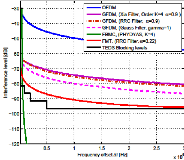
Figure 3.17: Effective interference powers [in dBc] of 1.4 MHz band of different multi-c waveforms versus 25KHz TEDS reception mask.
