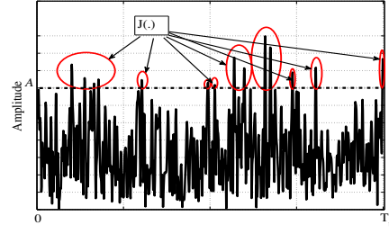
Fig. 1. Illustration of the cost function in TR-GP method.
