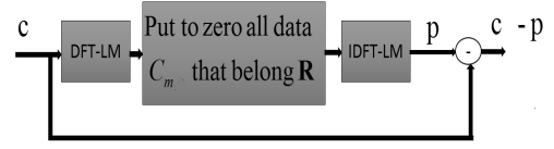
Fig. 3. Digital Frequency Domain Filtering scheme.
