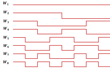
Figure 4: Walsh-Hadamard functions.
