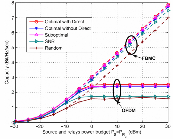
Fig. 2. Achieved capacity vs available power budget with P_S = P_{R_m} when I_{th} = -30 dBm. OFDM based system is plotted by the solid lines while the dashed ones represent the FBMC based systems.
