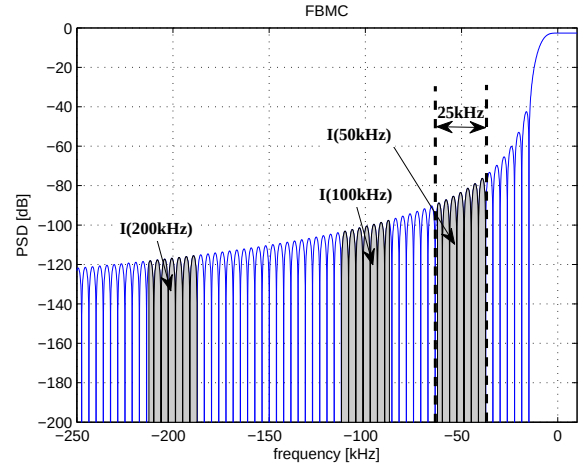
Fig. 4. : Effective interference levels of 1.4 MHz-LTE (73 active subcarriers) in 25 kHz-TEDS band, FBMC case
