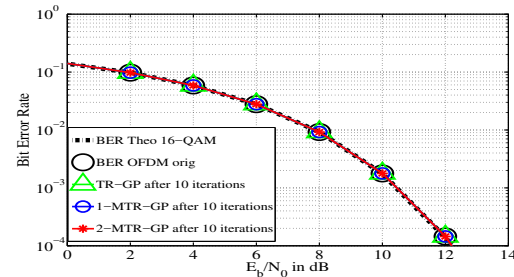
Fig. 7. BER performance of the signal before and after PAPR reduction.
