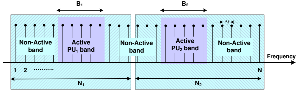
Figure 3.6: Frequency distribution with two active PU bands.
