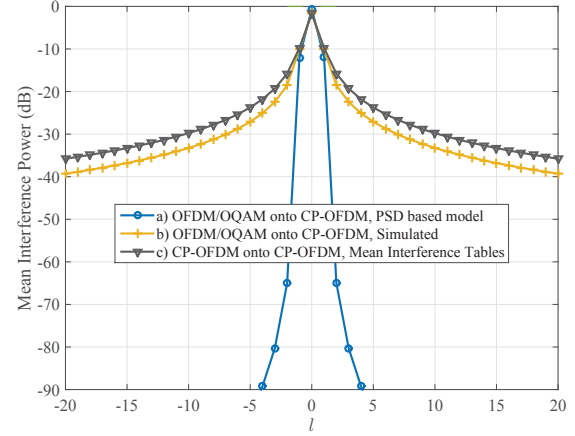
Fig. 5: Comparison between interference values obtained with (a) OFDM/OQAM onto CP-OFDM with PSD-based model, (b) OFDM/OQAM onto CP-OFDM through numerical simulation, and (c) CP-OFDM onto CP-OFDM with mean interference tables [17].
