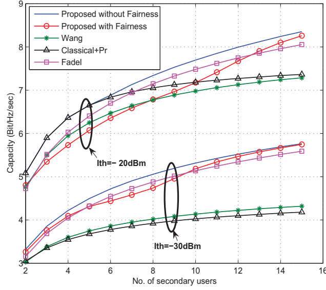
Figure 3.11: Achieved capacity vs No. of SUs when N = 128 subcarriers, \overline{P_m} = 1mWatt , B^1 = B^2 = 10 MHz, and R_{min} = 20 Mbits/sec.
