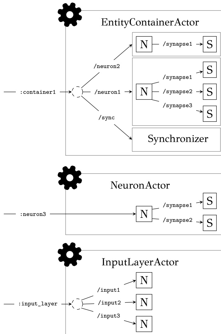
Figure 3.1: In N2S3, a network is organized in specialized actors that may contain one or more network entities. Such entities could be, for instances, neurons, inputs or any other. Each entity can be queried thank to its URL.
